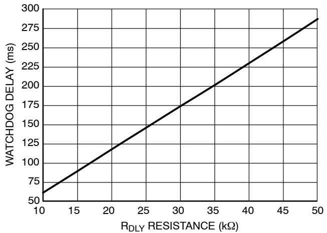
Figure 38. Watchdog Delay vs. RDLY Resistance
