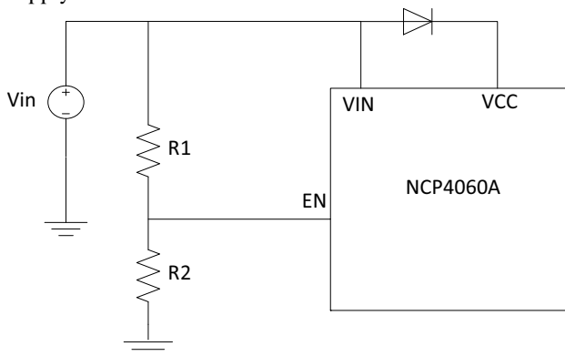
Figure 40. Input Blocking Diode for V_{EXT} > V_{CC}
