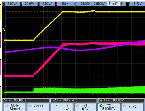
Figure 22. Start-Up Transition at 6A Load
