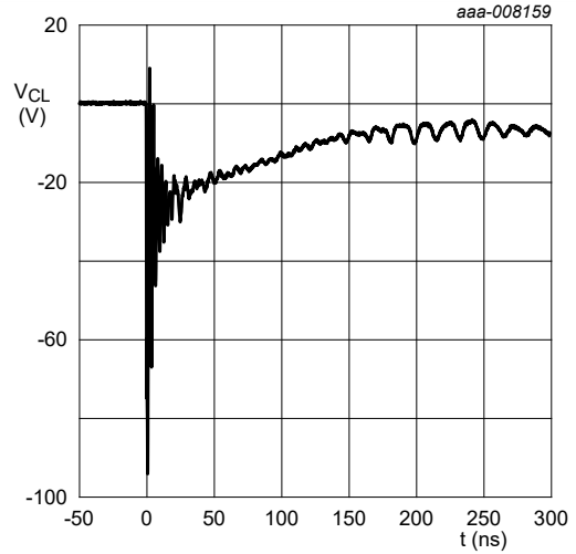
Fig. 5. Clamped -8 kV pulse waveform (IEC 61000-4-2 network)
