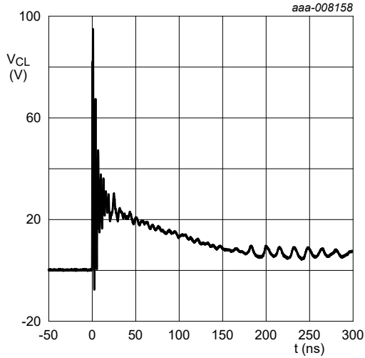
Fig. 4. Clamped +8 kV pulse waveform (IEC 61000-4-2 network)
