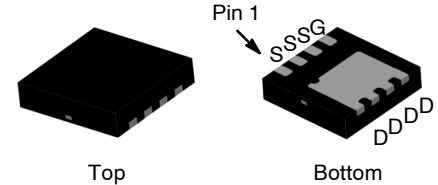
WDFN8 3.3x3.3, 0.65P CASE 511DH
