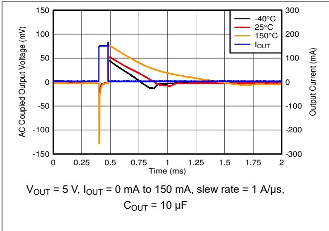
Figure 6-19. Load Transient, No Load to 150-mA
