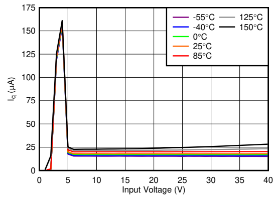
Figure 6-26. Quiescent Current ( I_Q ) vs V_{IN} V_{OUT} = 5\text{ V}
