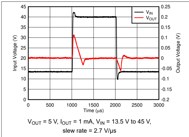
Figure 6-13. Line Transients
