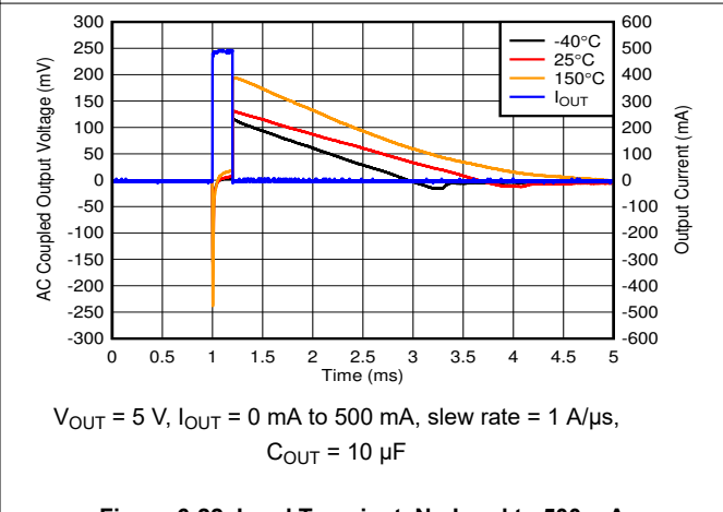
Figure 6-22. Load Transient, No Load to 500 mA
