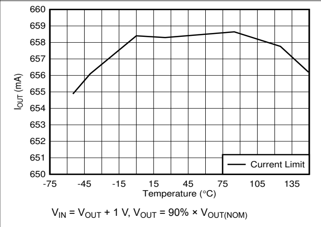
Figure 6-24. Output Current Limit vs Temperature
