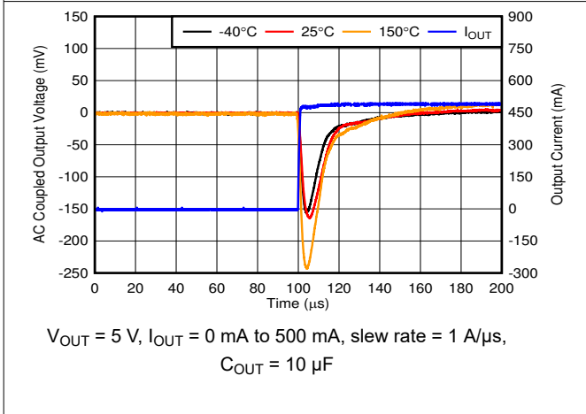
Figure 6-23. Load Transient, No Load to 500-mA Rising Edge
