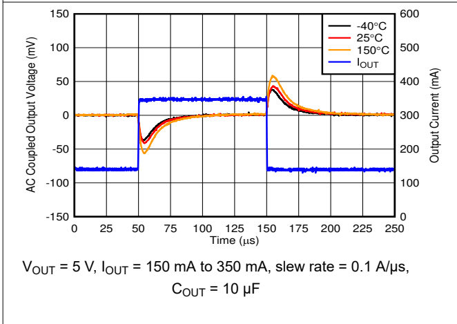
Figure 6-21. Load Transient, 150-mA to 350-mA
