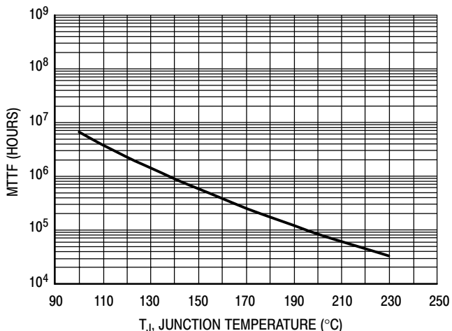
This above graph displays calculated MTTF in hours when the device is operated at V_{DD} = 28 \text{ Vdc} , P_{out} = 35.5 \text{ W CW} , and \eta_D = 57\% . MTTF calculator available at http://www.freescale.com/rf . Select Software & Tools/Development Tools/Calculators to access MTTF calculators by product.
