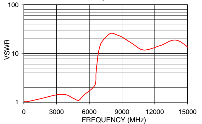
LFCN-5850+ VSWR
