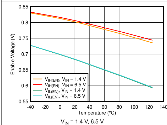
Figure 6-39. Enable Threshold vs Temperature
