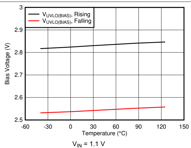
Figure 6-38. V_{BIAS} UVLO vs Temperature
