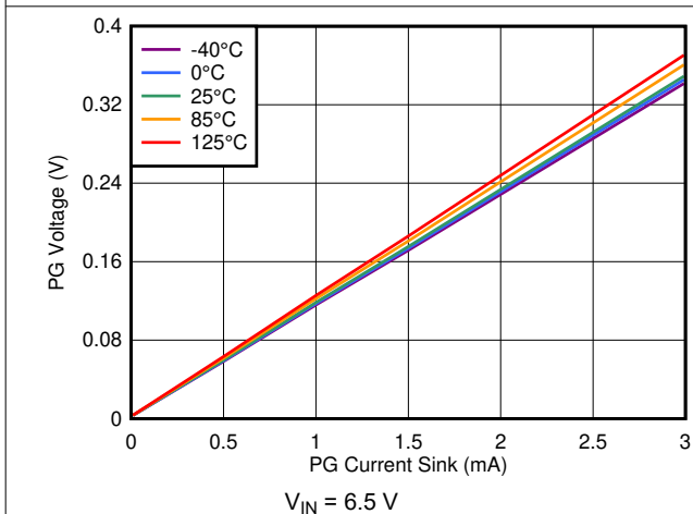
Figure 6-41. PG Voltage vs PG Current Sink
