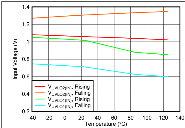
Figure 6-37. V_{IN} UVLO vs Temperature
