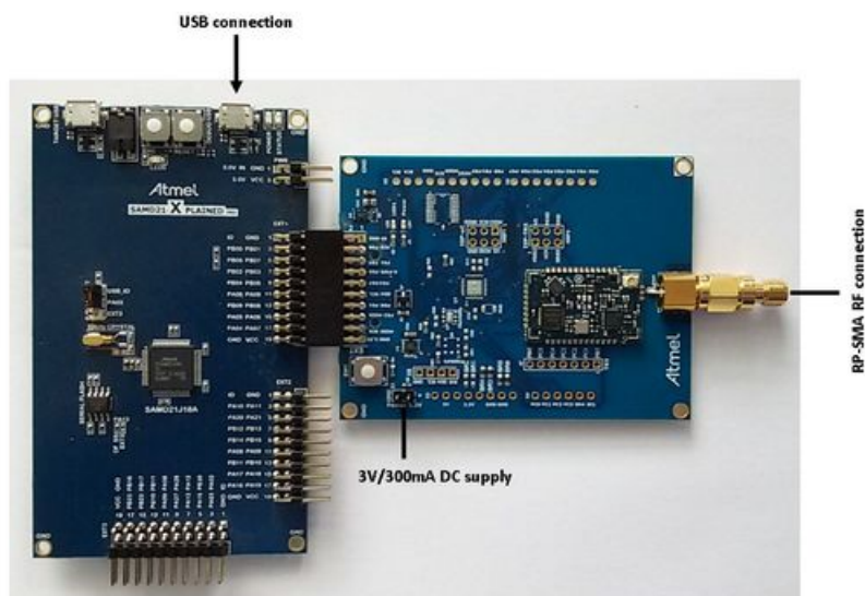
Figure 3-8. ATA8520-EK3-F
