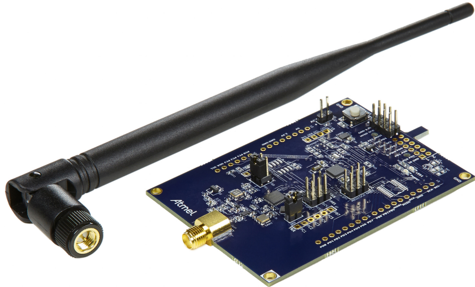
Figure 3-2. ATA8520-EK1-E
