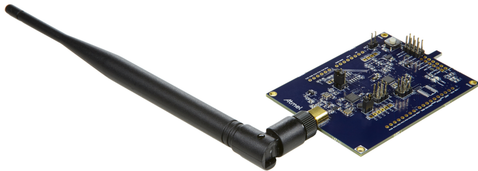
Figure 3-3. ATA8520-EK2-E
