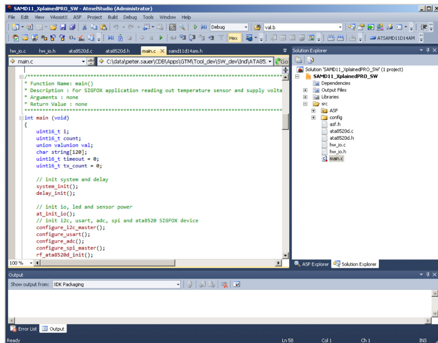
Figure 4-1. Atmel Studio 6
