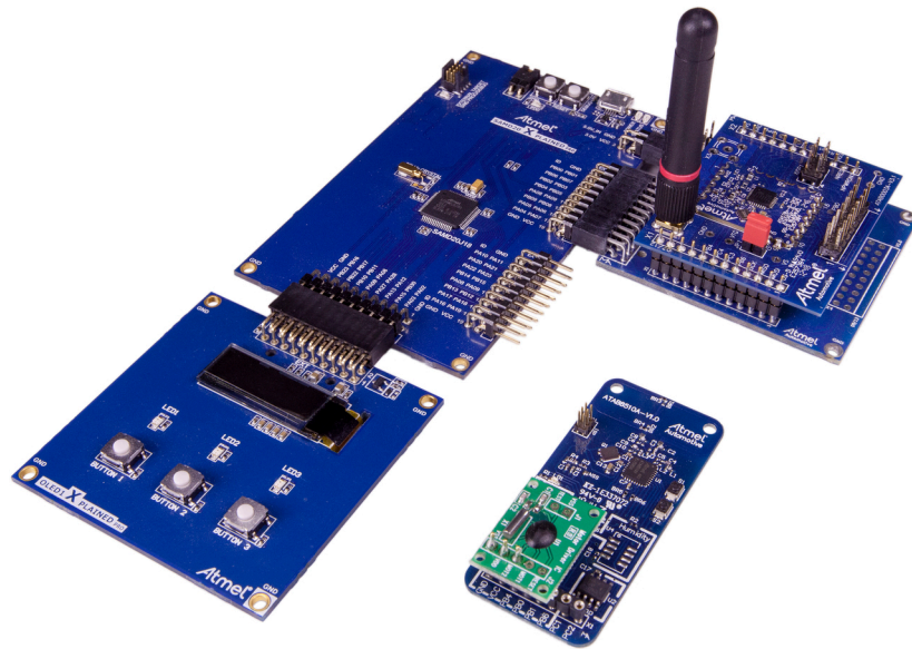
Figure 3-1. ATA8510-EK1
