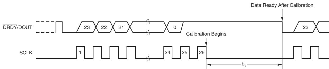
Figure 8-11. Offset-Calibration Timing
