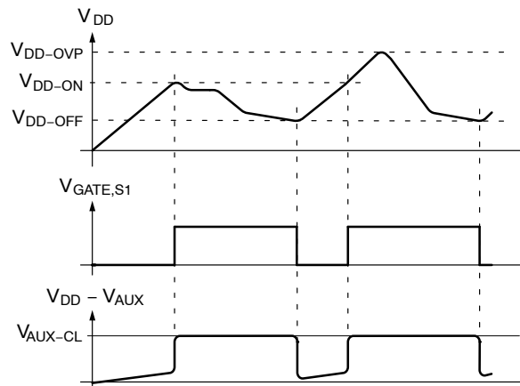
Figure 28. Start Up Sequence With AUX Controlling
