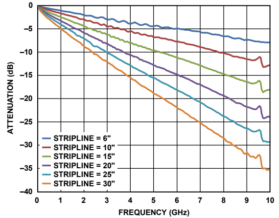
Figure 52. Insertion Loss of 50 \Omega Striplines on FR4
