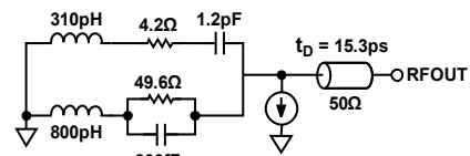
Figure 93. Equivalent Output Circuit to Pin RFOUT
