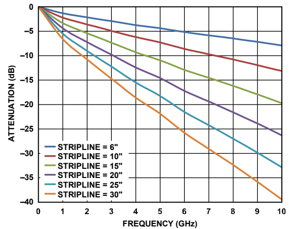
Figure 53. Insertion Loss of 50 \Omega Microstrips on FR4
