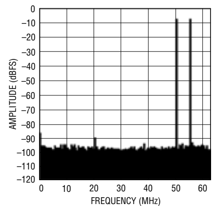
LTM9011-14, 125MSPS, 2-Tone FFT, f IN = 70MHz and 75MHz
