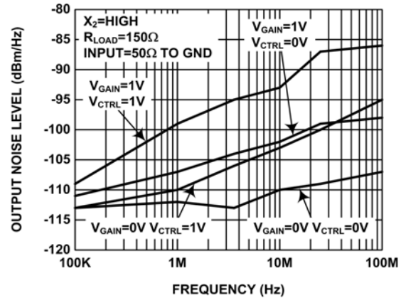
FIGURE 8. OUTPUT NOISE
