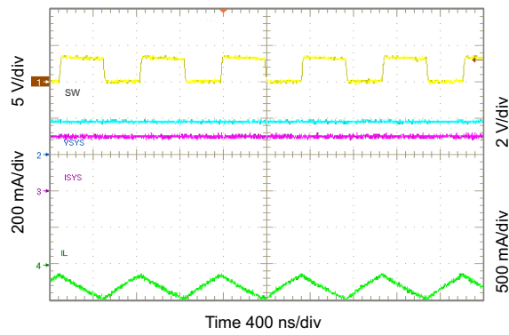
Figure 10-30. Light Load Operation Showing SW
