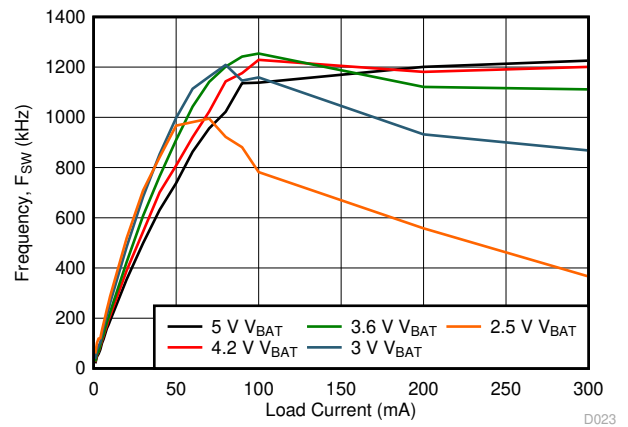
Figure 10-23. 1.8 V SYS Switching Frequency vs Load Current
