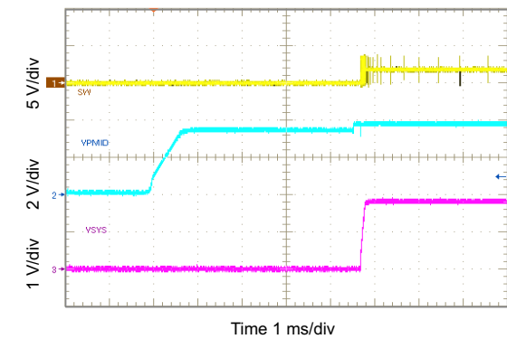
Figure 10-41. Startup Showing SS on SYS in PWM Mode
