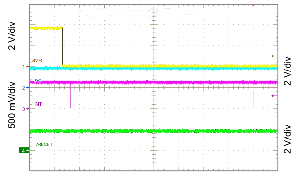
Figure 10-60. PG Functions as Shifted MR Output
