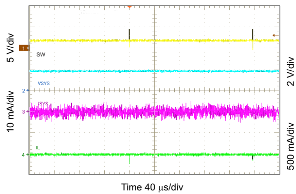
Figure 10-22. 3.3 V SYS Line Regulation
