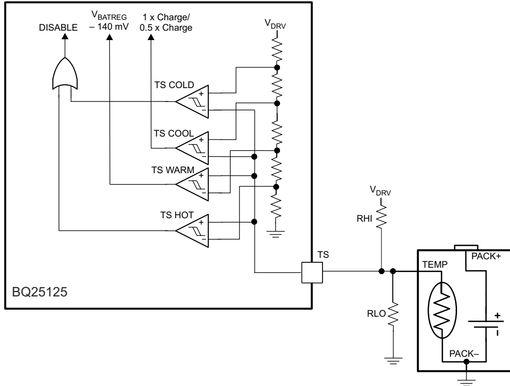
Figure 9-4. TS Circuit
