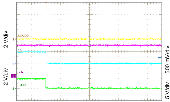
Figure 10-59. PG Functions as Shifted MR Output
