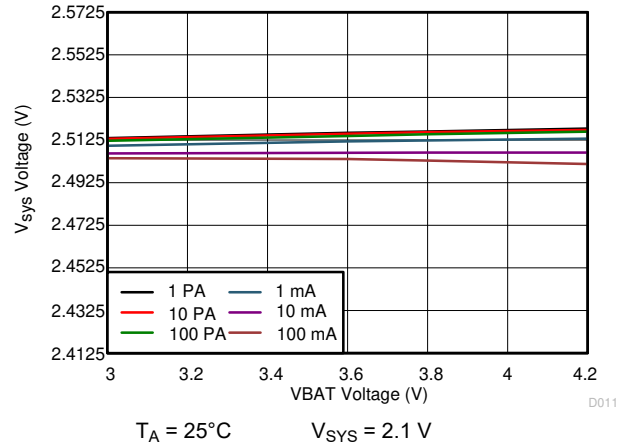
Figure 10-21. 2.1 V SYS Line Regulation
