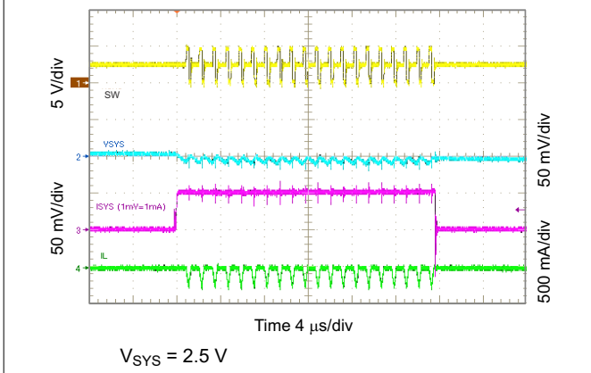
Figure 10-34. 2.5 V SYS Load Transient, 0 to 50 mA
