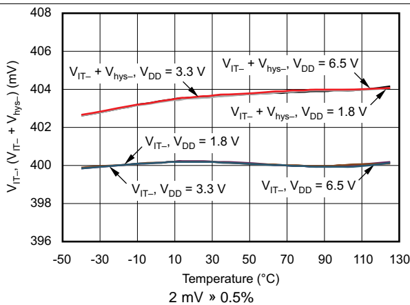
Figure 16. TPS386000-Q1 SENSE4L Threshold Voltage vs Temperature
