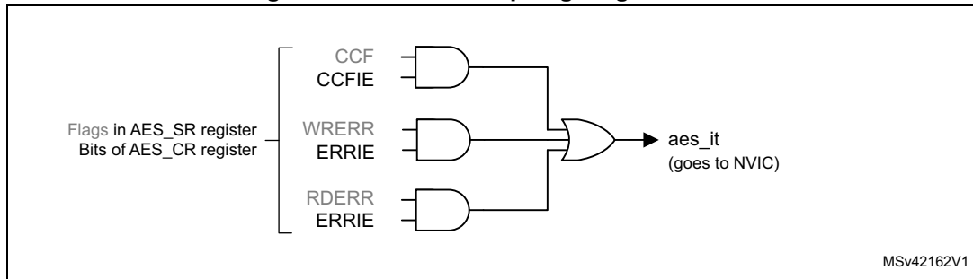
Figure 103. AES interrupt signal generation
