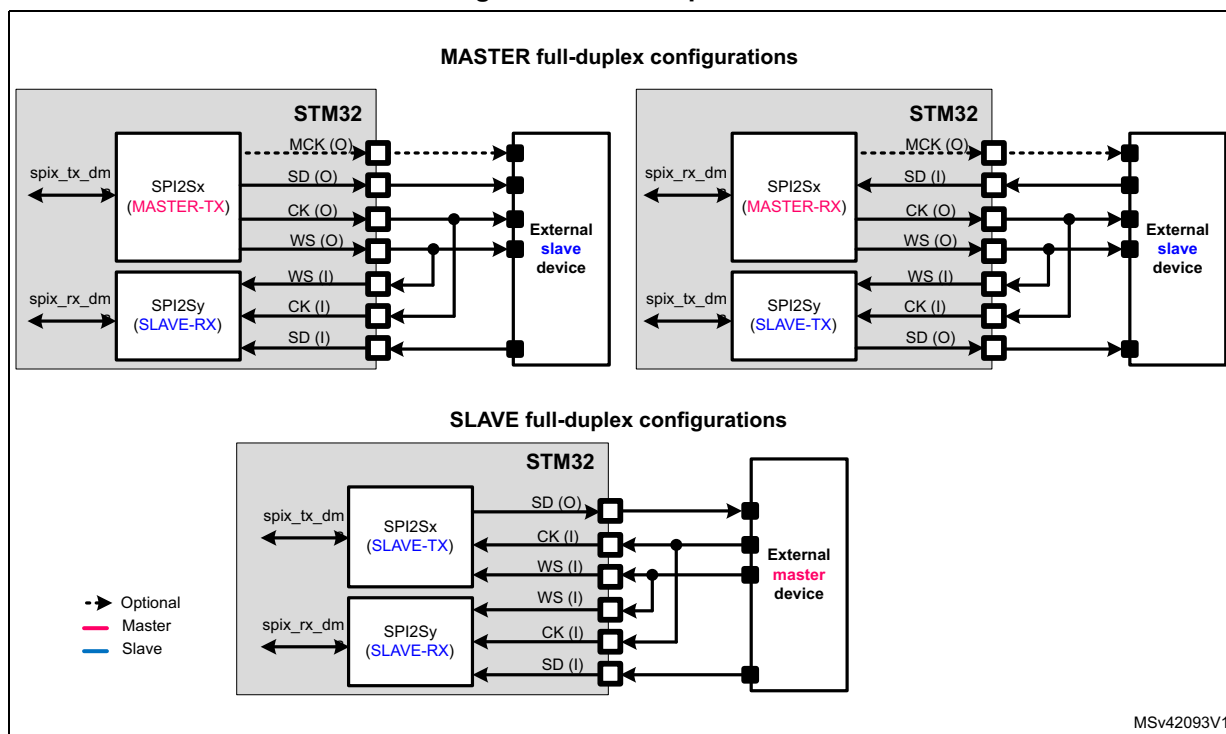
Figure 293. Full-duplex communication
