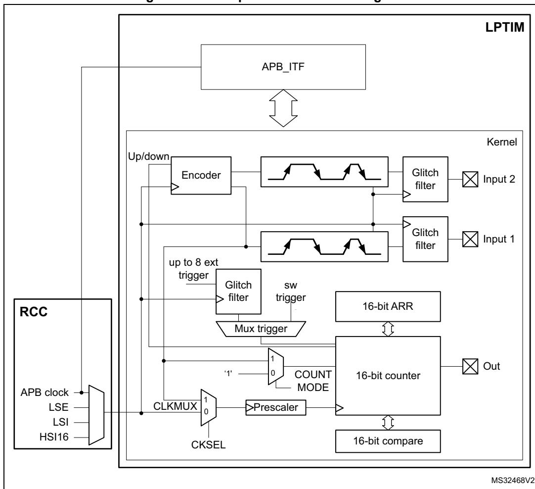
Figure 200. Low-power timer block diagram
