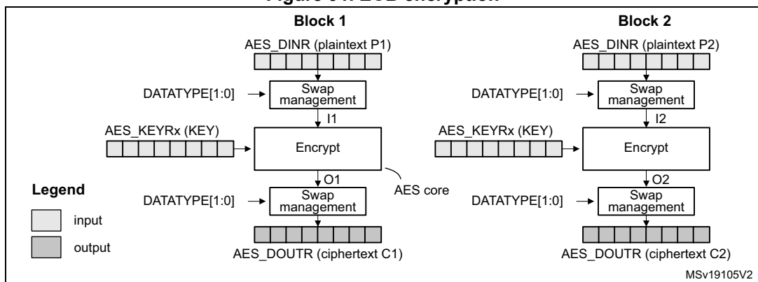
Figure 91. ECB encryption
