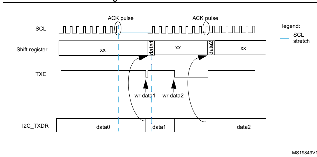
Figure 217. Data transmission
