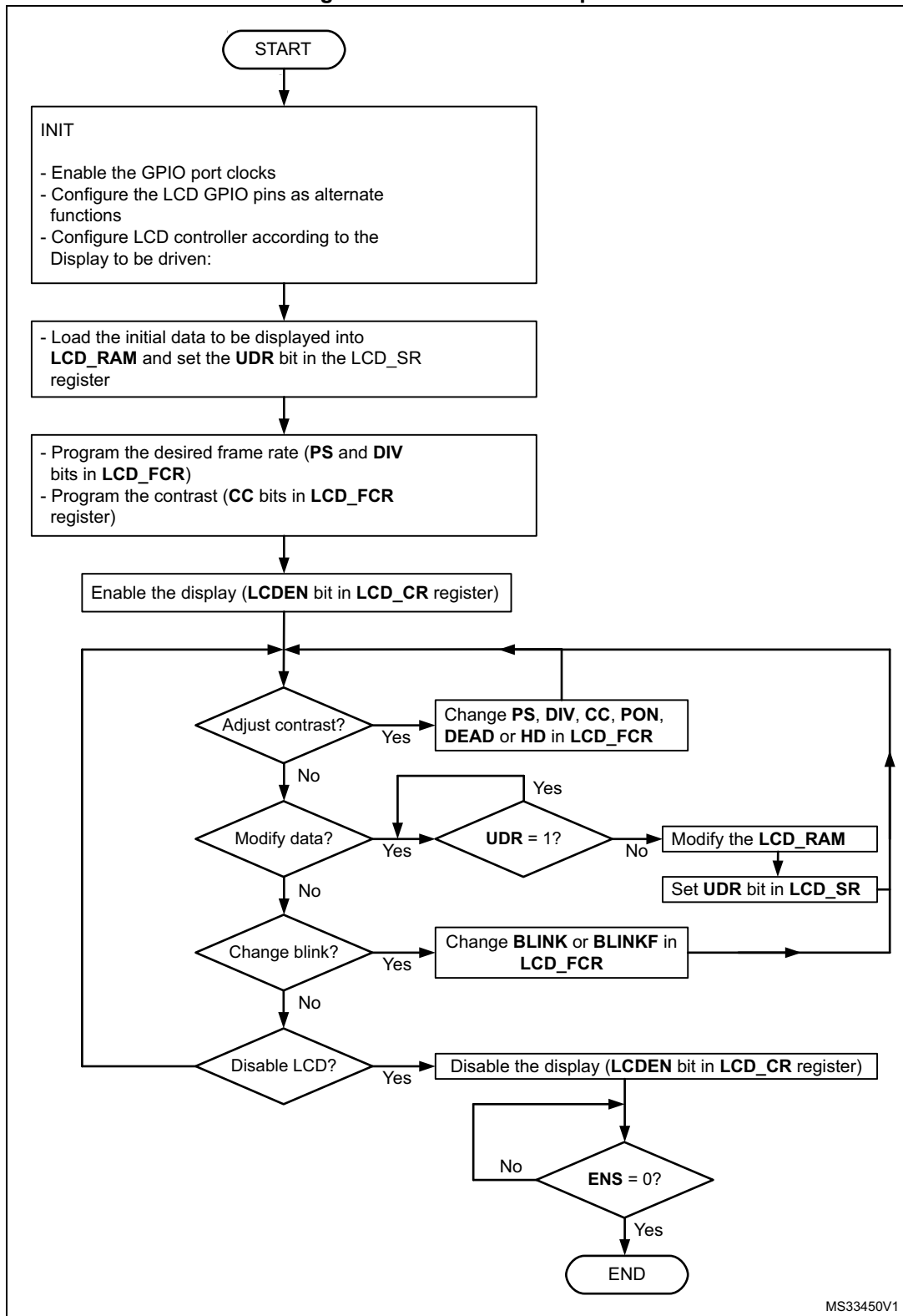
Figure 78. Flowchart example
