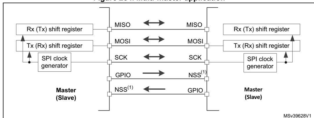
Figure 284. Multi-master application
