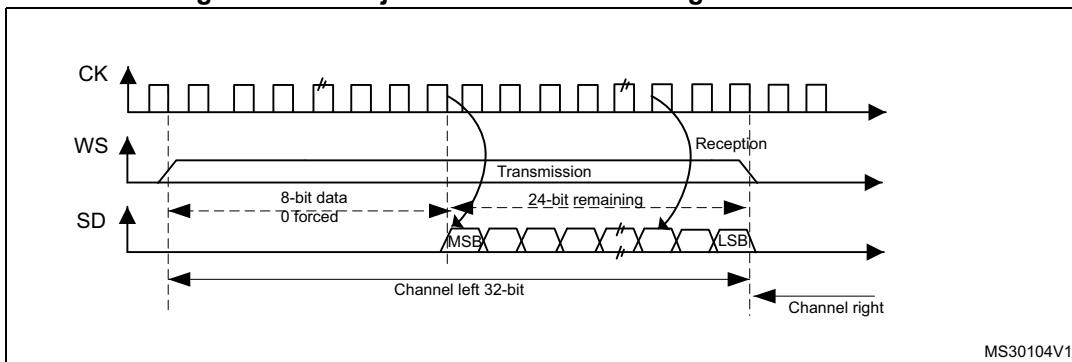
Figure 304. LSB justified 24-bit frame length with CPOL = 0
