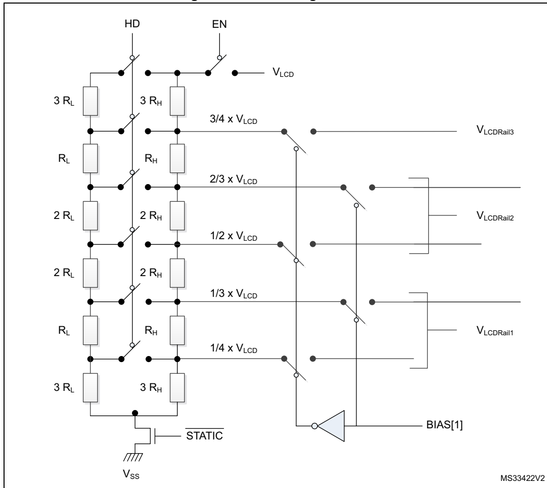
Figure 75. LCD voltage control
