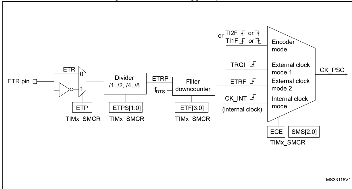
Figure 174. External trigger input block
