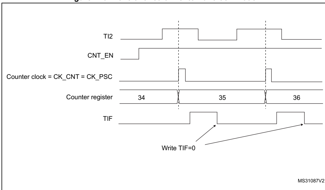
Figure 173. Control circuit in external clock mode 1
