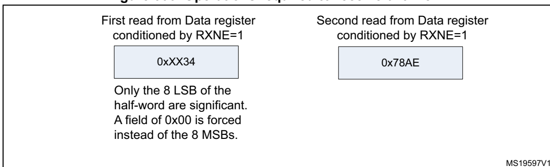
Figure 306. Operations required to receive 0x3478AE
