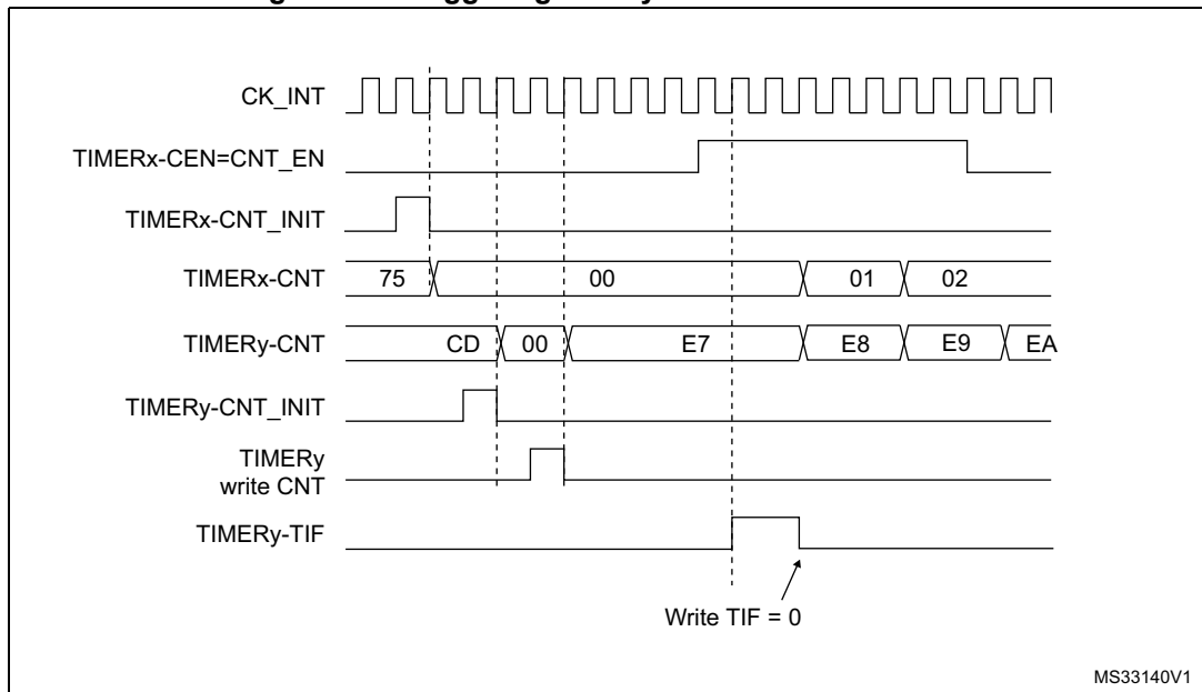
Figure 150. Triggering timer y with Enable of timer x
