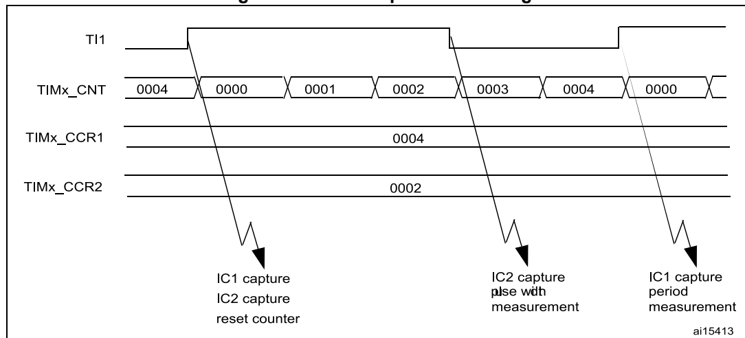
Figure 134. PWM input mode timing
