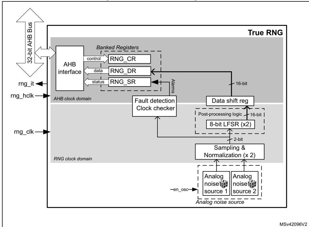
Figure 104. RNG block diagram
