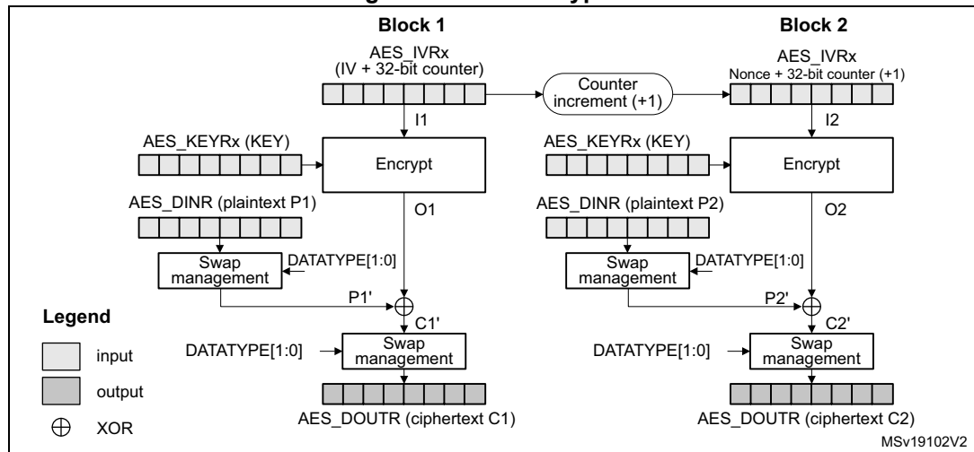
Figure 98. CTR encryption
