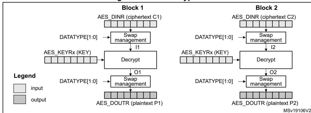
Figure 92. ECB decryption
