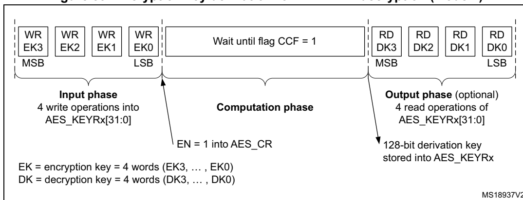
Figure 89. Encryption key derivation for ECB/CBC decryption (Mode 2)
