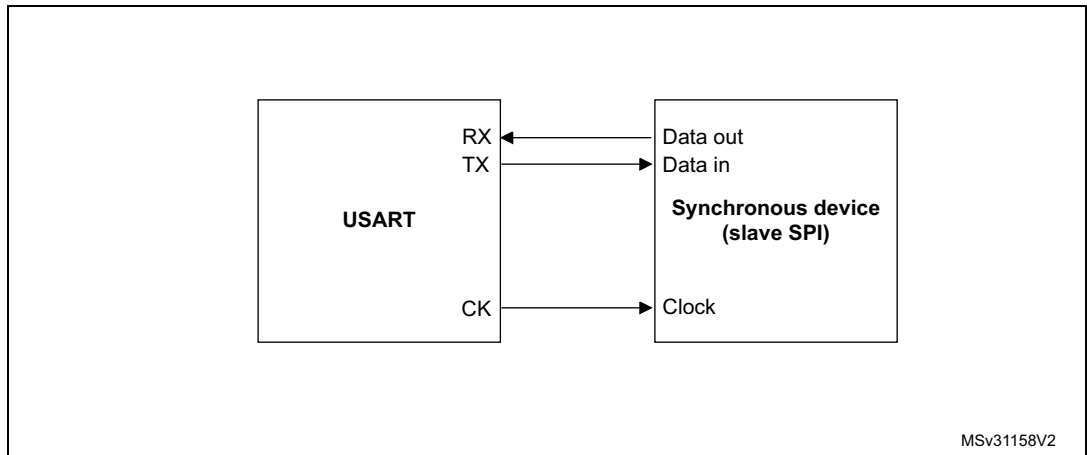
Figure 253. USART example of synchronous transmission
