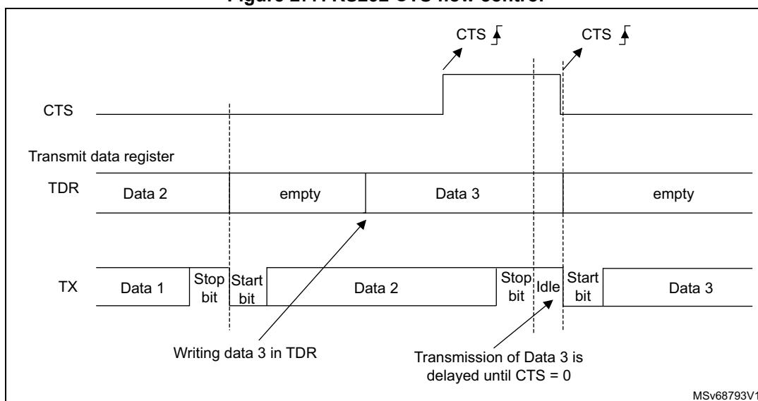
Figure 277. RS232 CTS flow control
