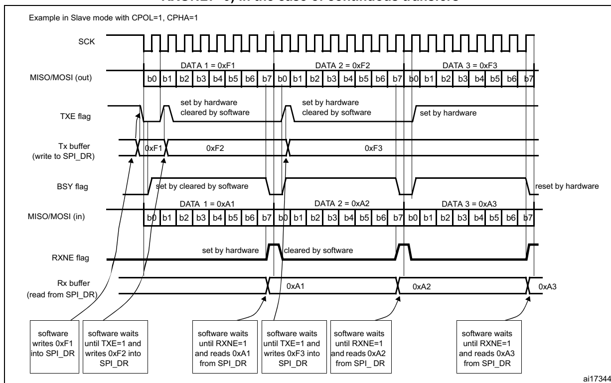
Figure 288. TXE/RXNE/BSY behavior in slave / full-duplex mode (BIDIMODE=0, RXONLY=0) in the case of continuous transfers
