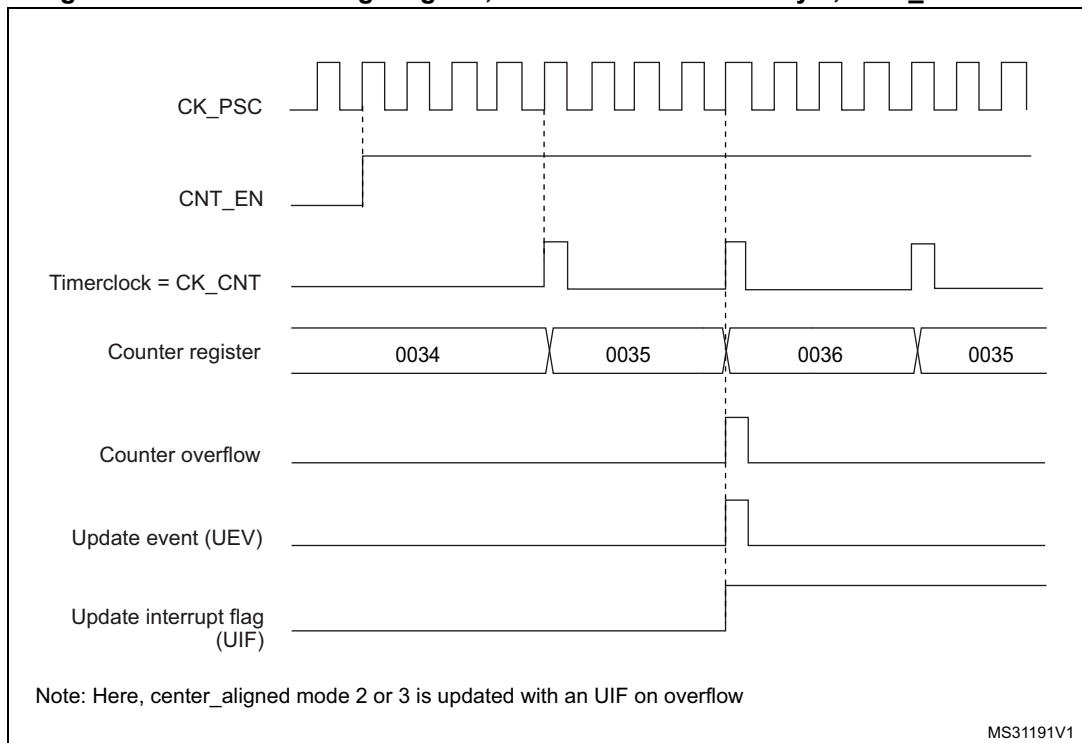
Figure 122. Counter timing diagram, internal clock divided by 4, TIMx_ARR=0x36
