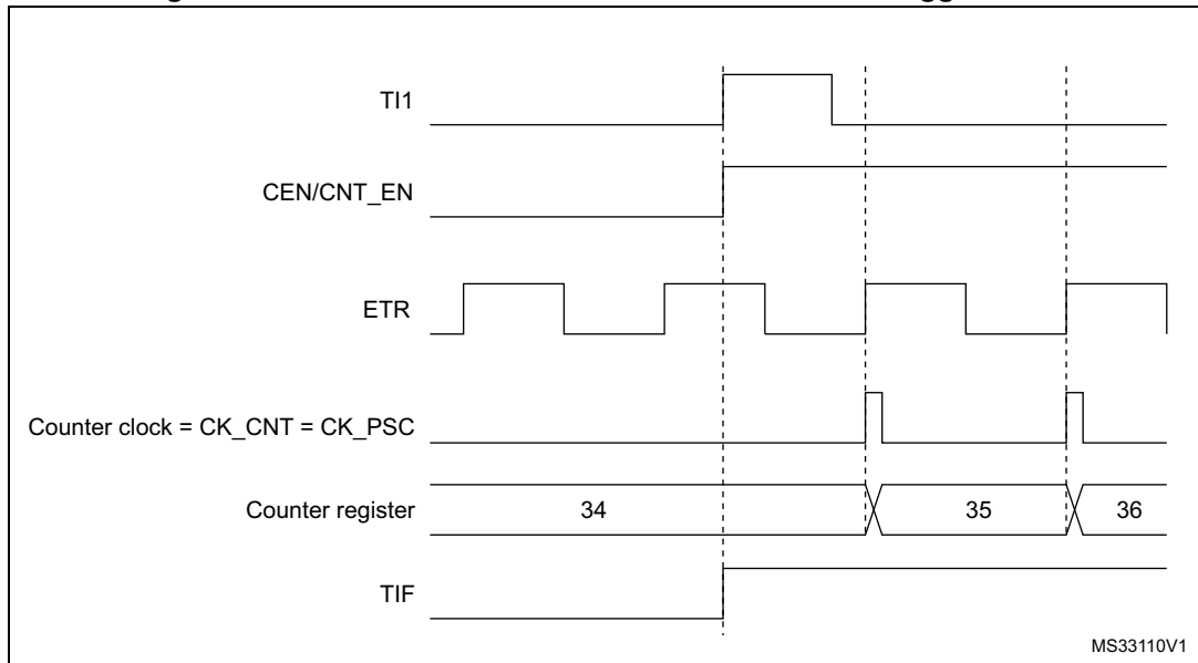
Figure 145. Control circuit in external clock mode 2 + trigger mode
