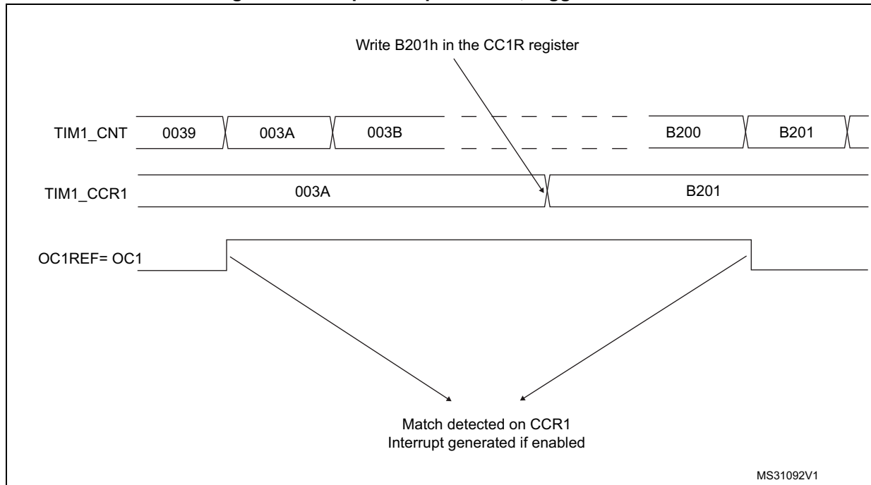
Figure 135. Output compare mode, toggle on OC1.
