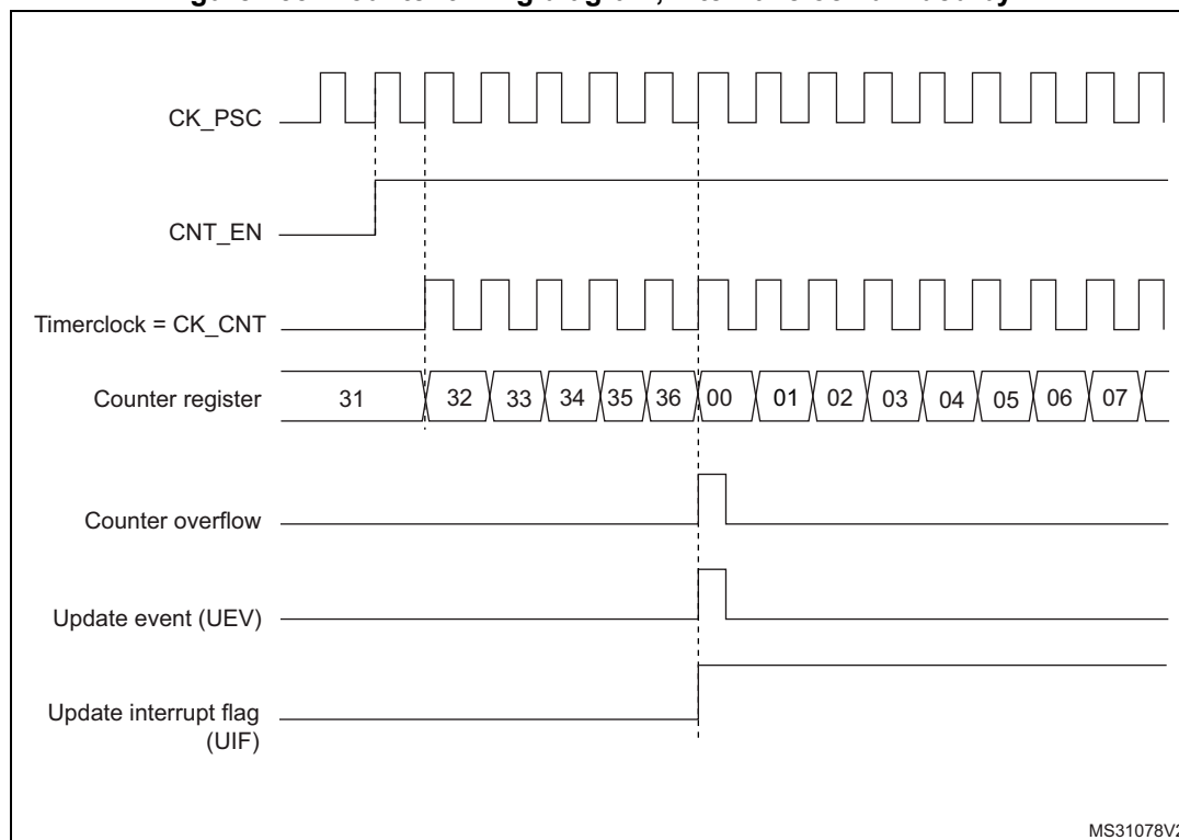
Figure 155. Counter timing diagram, internal clock divided by 1
