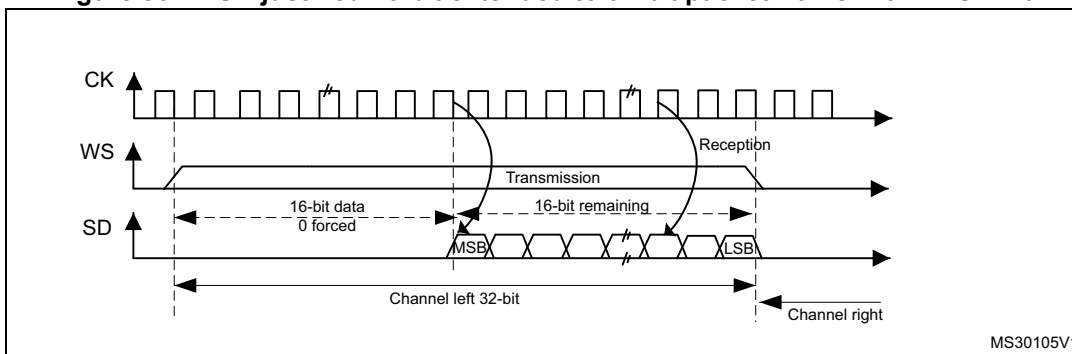
Figure 307. LSB justified 16-bit extended to 32-bit packet frame with CPOL = 0
