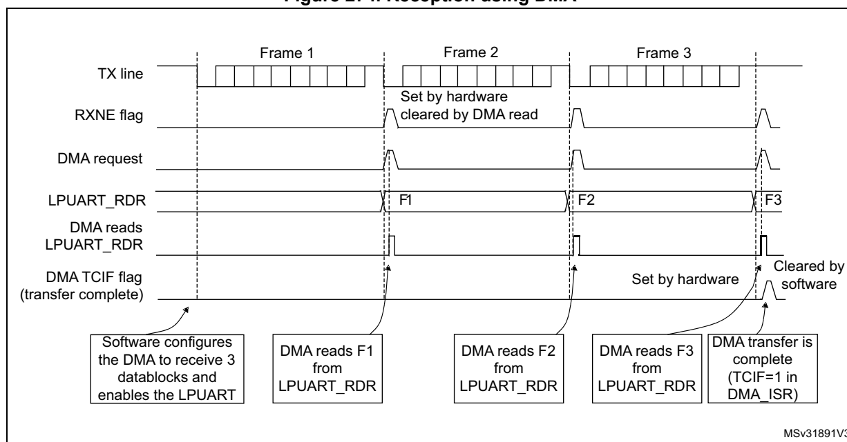
Figure 274. Reception using DMA
