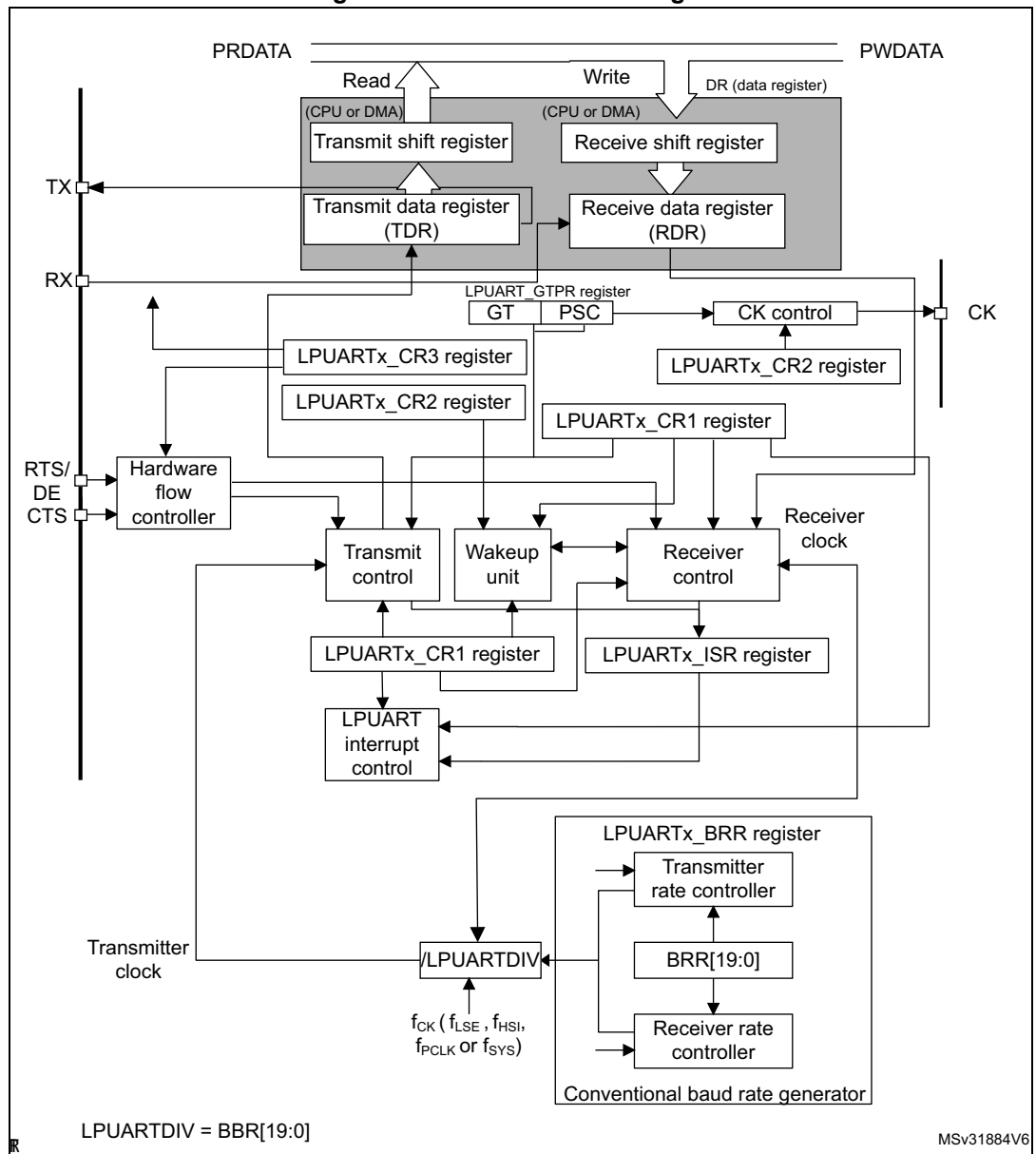
Figure 267. LPUART block diagram
