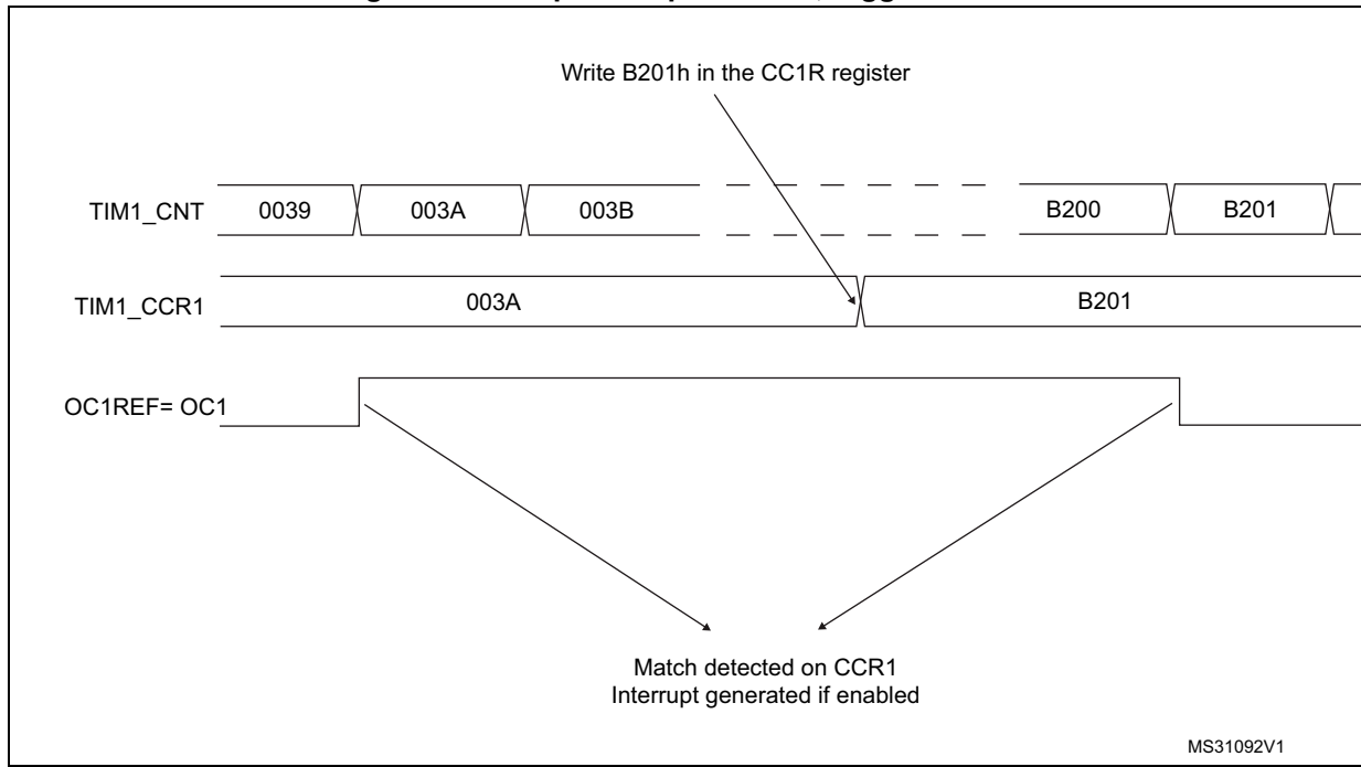
Figure 180. Output compare mode, toggle on OC1
