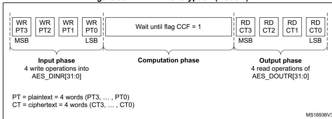
Figure 95. ECB/CBC encryption (Mode 1)
