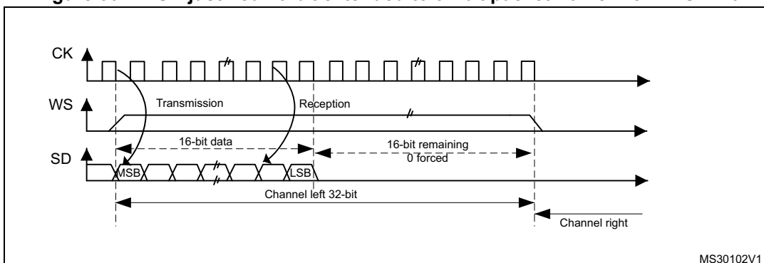
Figure 302. MSB justified 16-bit extended to 32-bit packet frame with CPOL = 0
