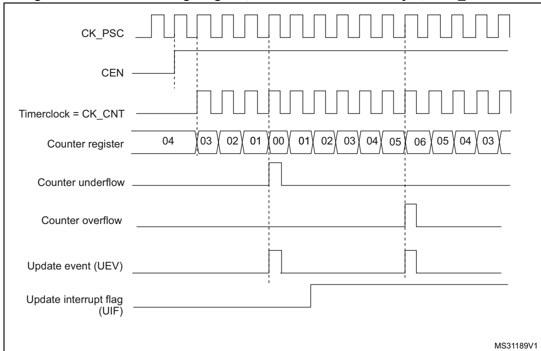
Figure 165. Counter timing diagram, internal clock divided by 1, TIMx_ARR=0x6
