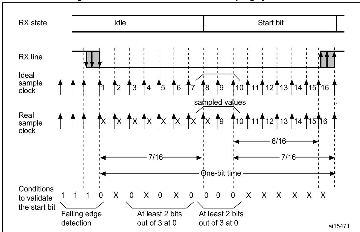
Figure 246. Start bit detection when oversampling by 16 or 8
