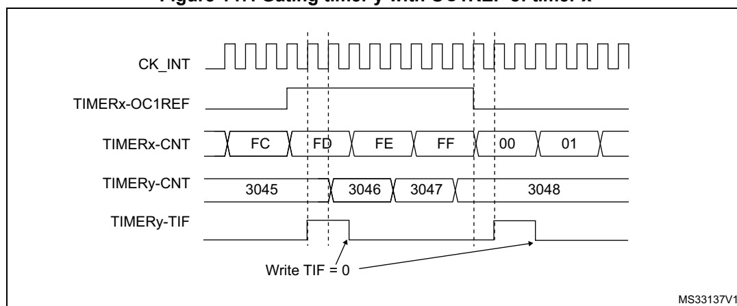
Figure 147. Gating timer y with OC1REF of timer x
