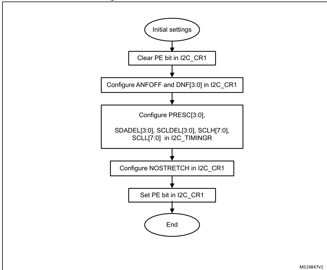
Figure 215. I2C initialization flow
