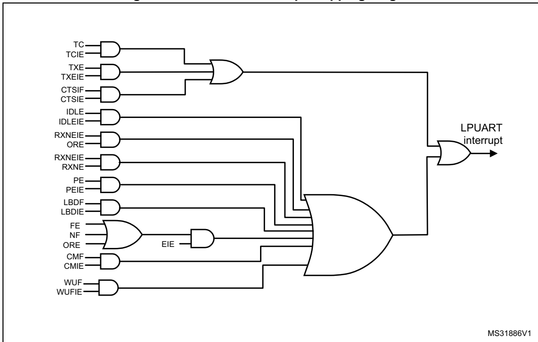
Figure 278. LPUART interrupt mapping diagram
