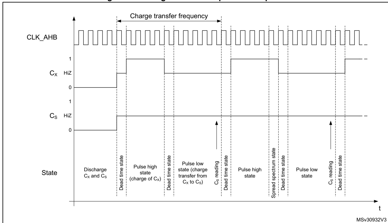
Figure 82. Charge transfer acquisition sequence
