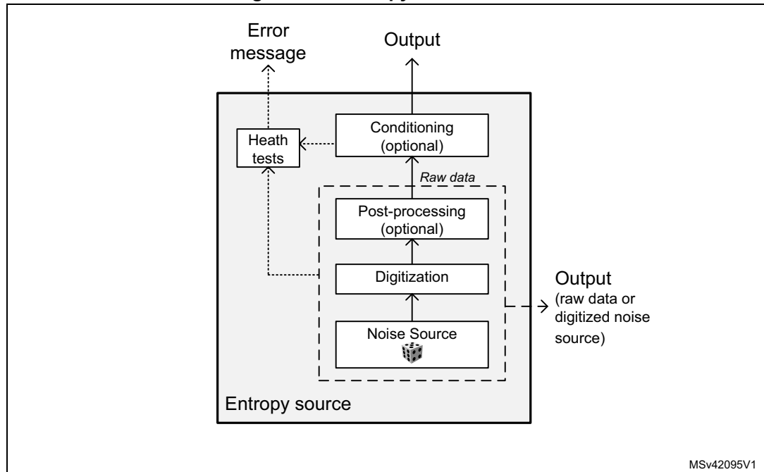
Figure 105. Entropy source model
