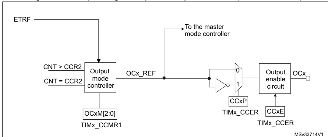
Figure 178. Output stage of capture/compare channel (channel 1 and 2)
