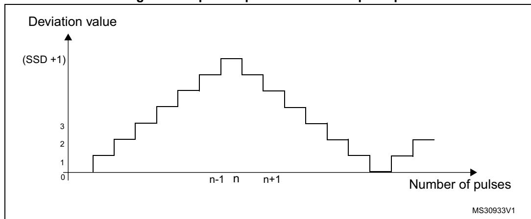
Figure 83. Spread spectrum variation principle
