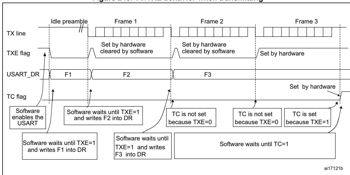
Figure 245. TC/TXE behavior when transmitting
