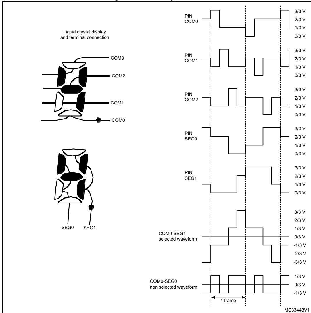
Figure 73. 1/4 duty, 1/3 bias
