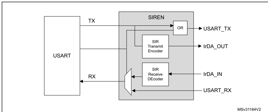
Figure 259. IrDA SIR ENDEC- block diagram
