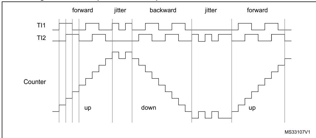
Figure 140. Example of counter operation in encoder interface mode
