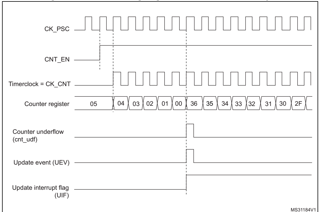
Figure 115. Counter timing diagram, internal clock divided by 1
