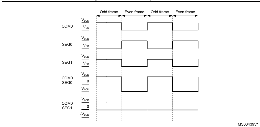
Figure 69. Static duty case 1
