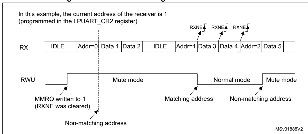
Figure 272. Mute mode using address mark detection
