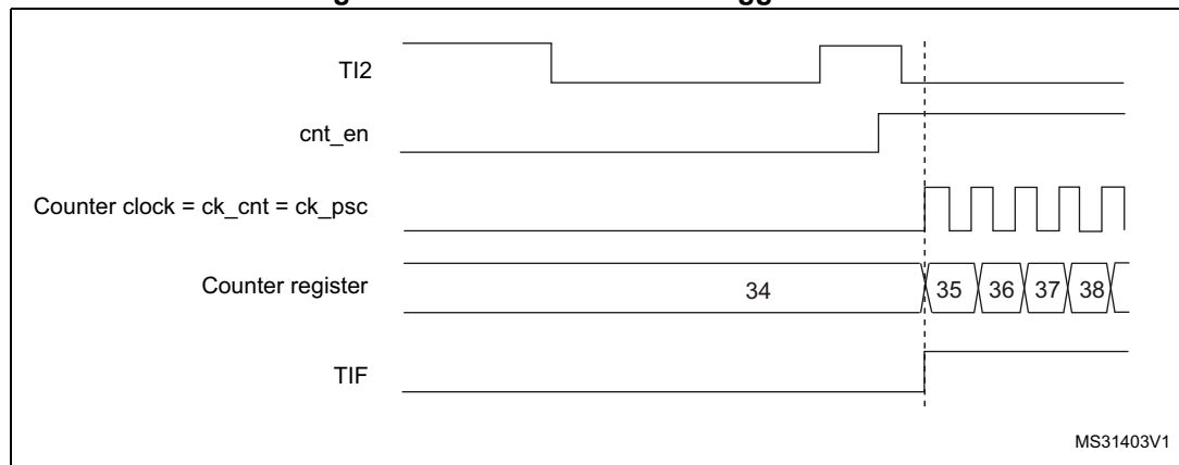
Figure 144. Control circuit in trigger mode
