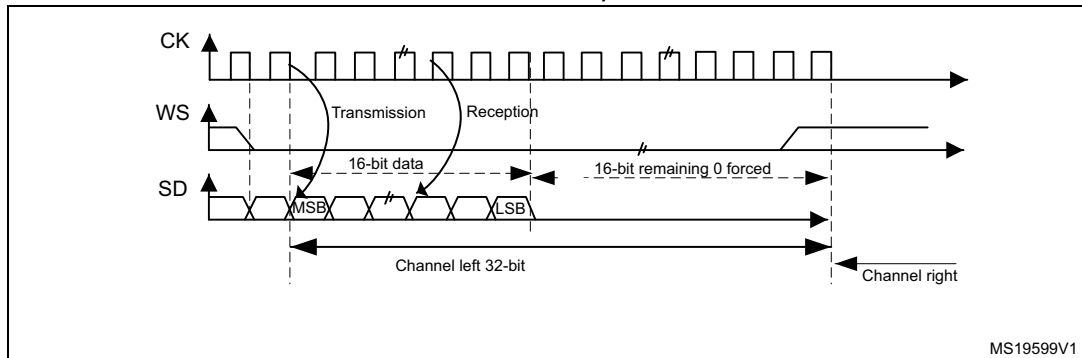
Figure 298. I 2 S Philips standard (16-bit extended to 32-bit packet frame with CPOL = 0)
