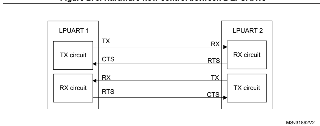
Figure 275. Hardware flow control between 2 LPUARTs
