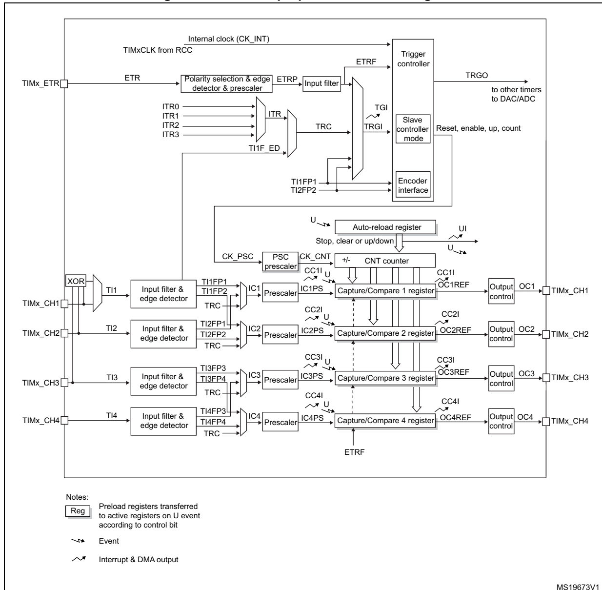
Figure 106. General-purpose timer block diagram
