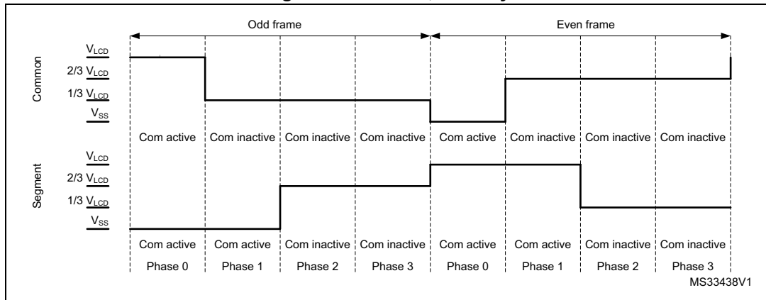
Figure 68. 1/3 bias, 1/4 duty
