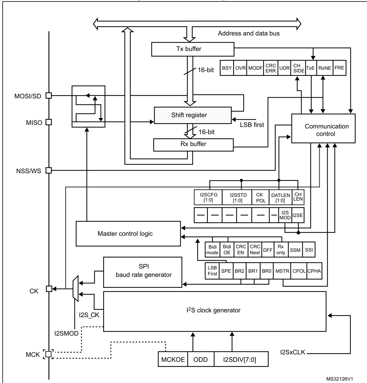
Figure 292. I 2 S block diagram
