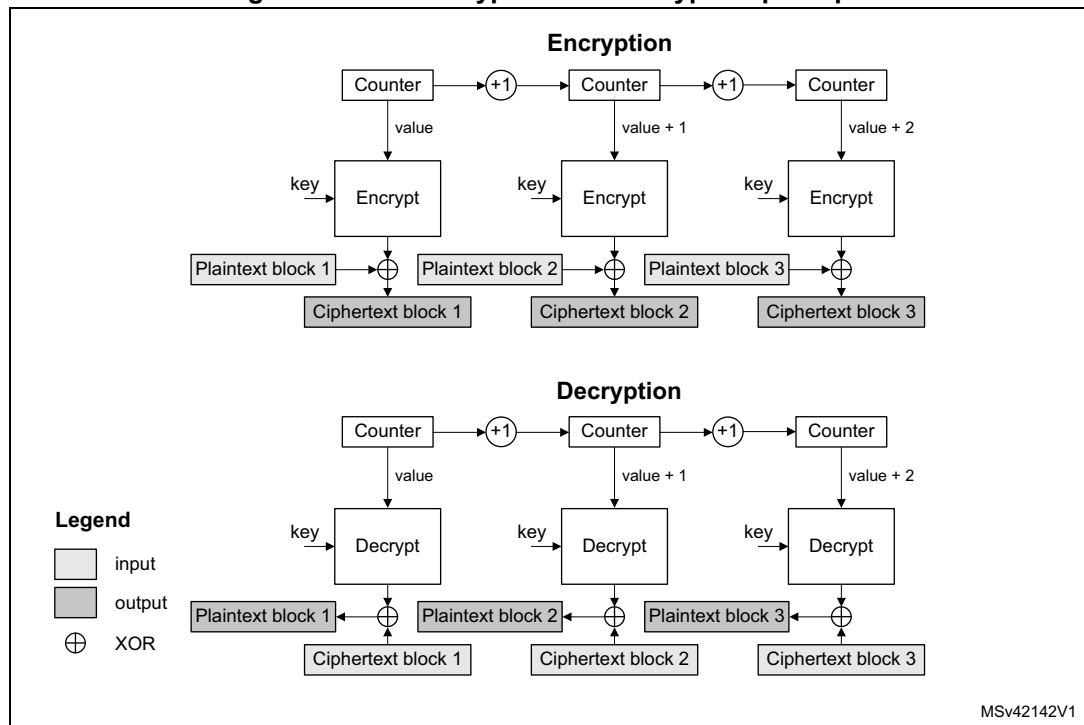
Figure 87. CTR encryption and decryption principle
