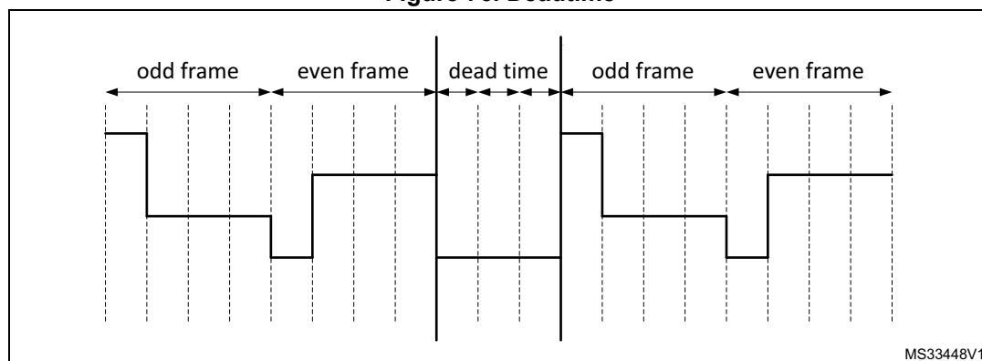
Figure 76. Deadtime
