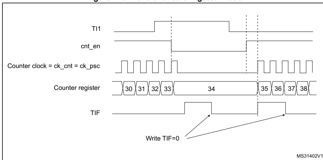
Figure 143. Control circuit in gated mode
