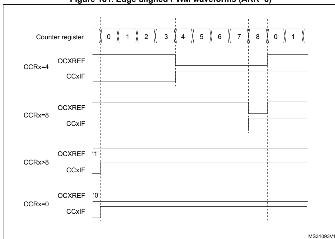
Figure 181. Edge-aligned PWM waveforms (ARR=8)
