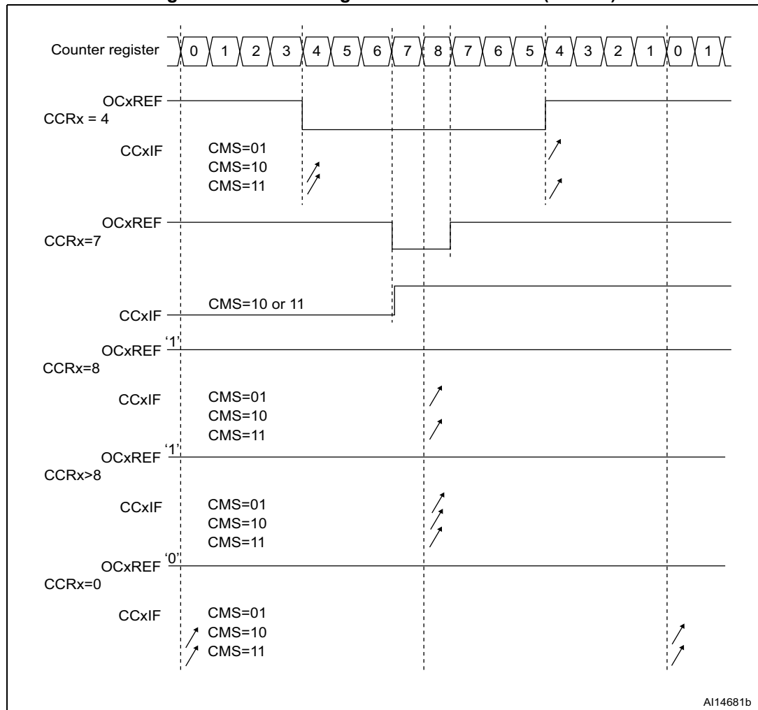
Figure 182. Center-aligned PWM waveforms (ARR=8)
