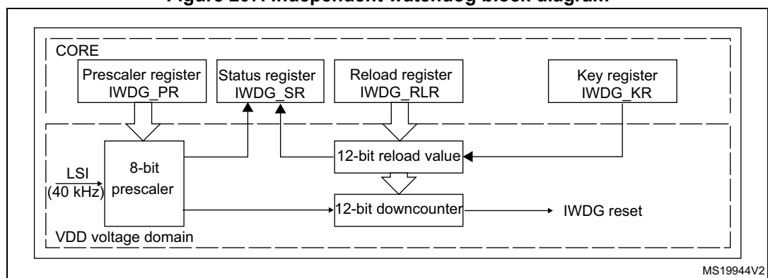
Figure 207. Independent watchdog block diagram
