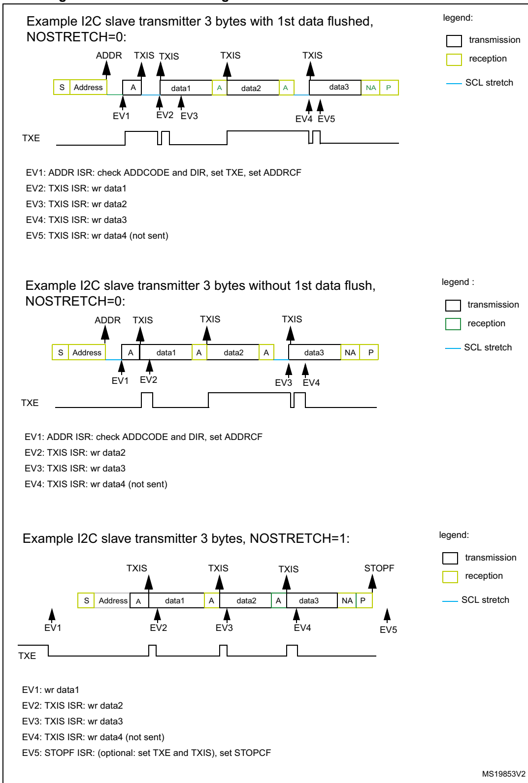
Figure 221. Transfer bus diagrams for I2C slave transmitter
