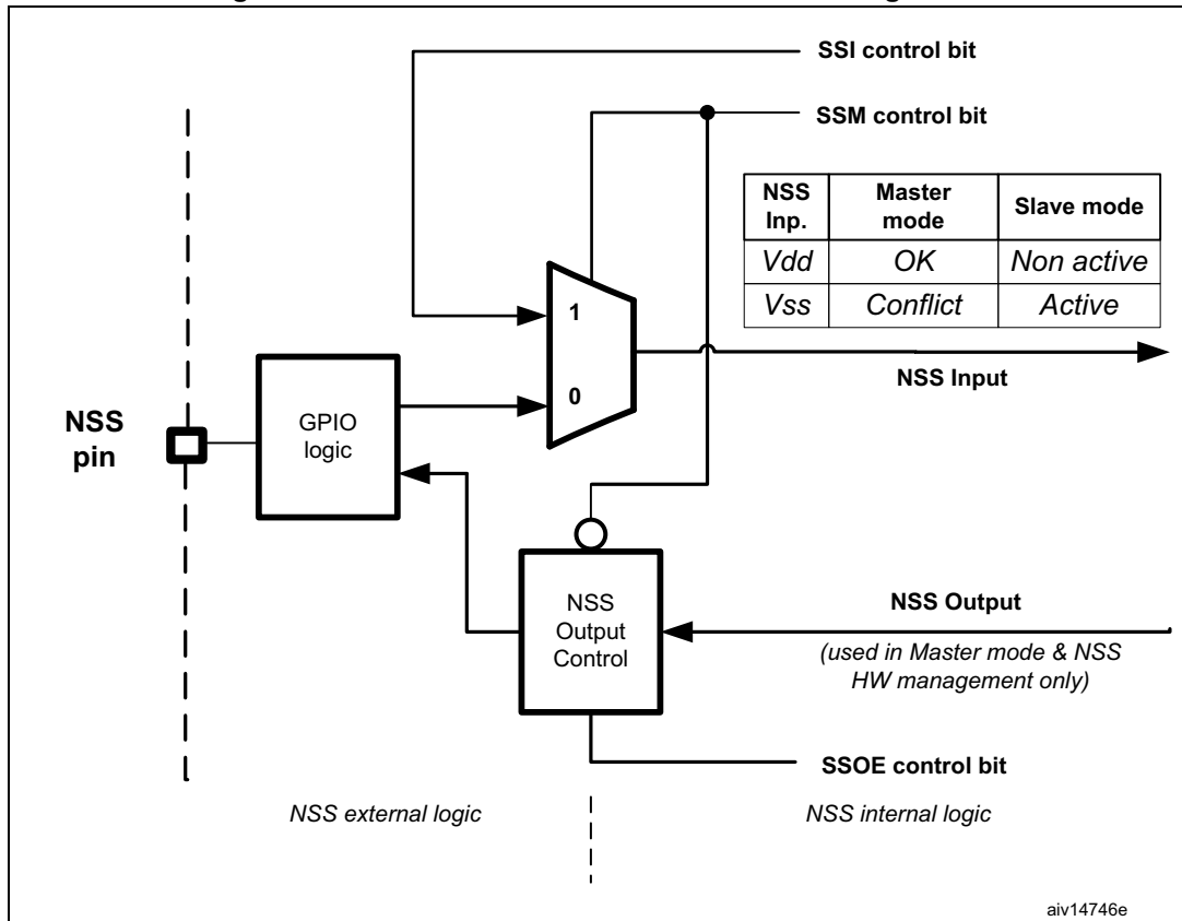
Figure 285. Hardware/software slave select management
