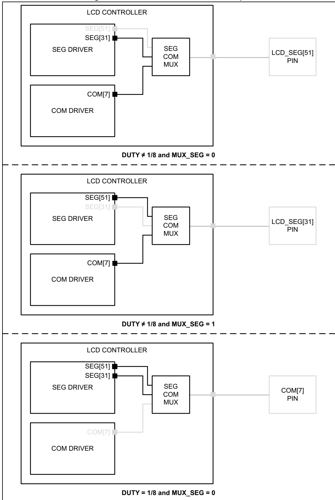
Figure 77. SEG/COM mux feature example
