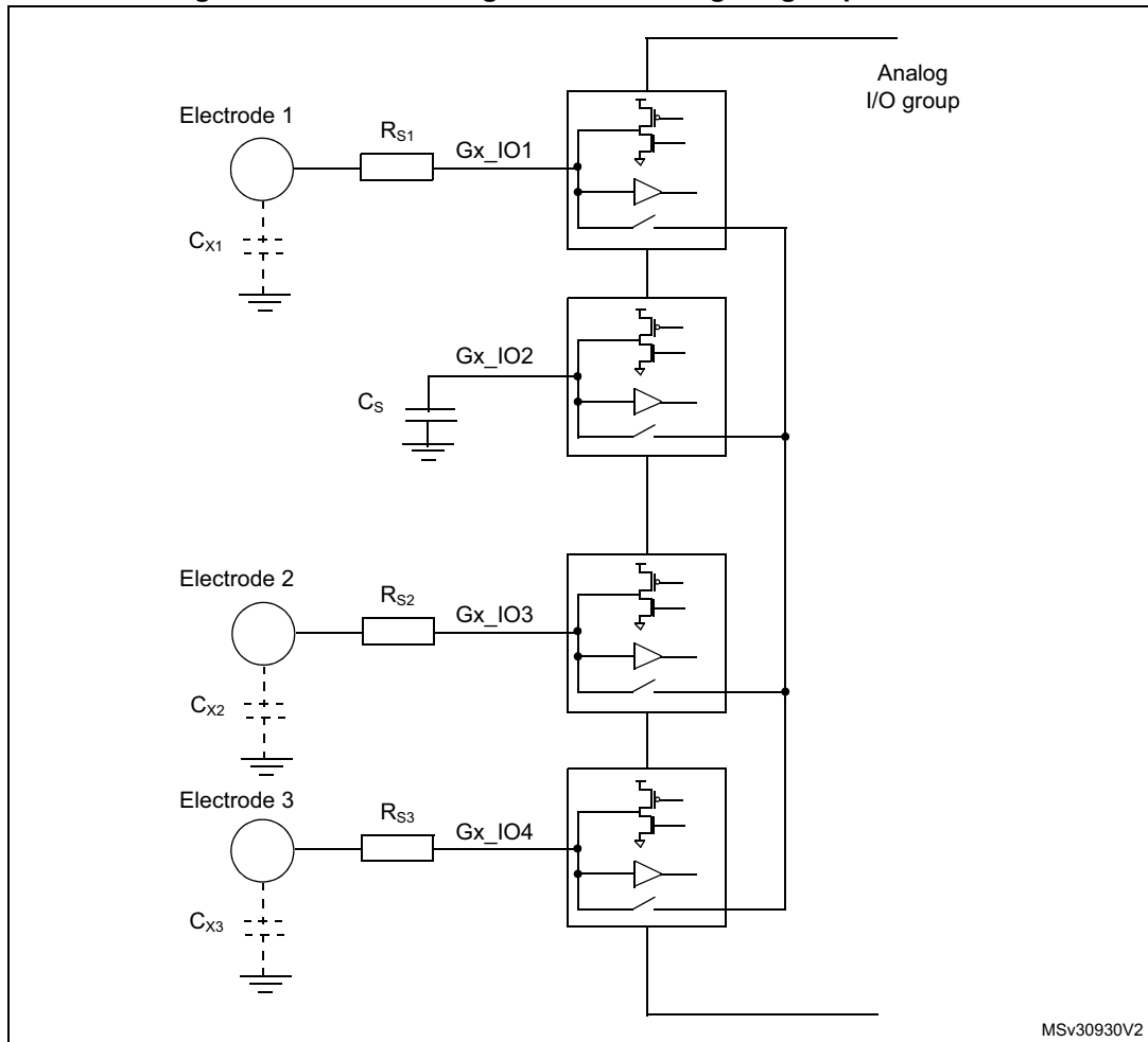
Figure 80. Surface charge transfer analog I/O group structure
