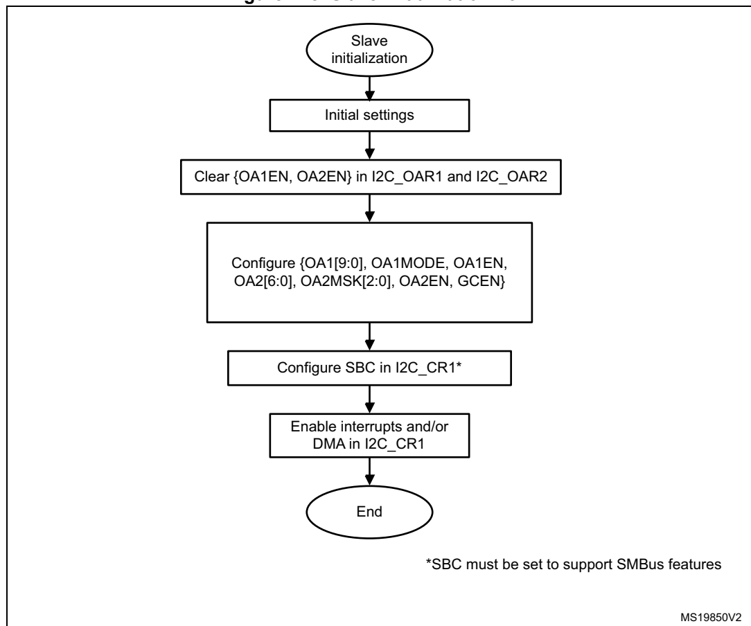
Figure 218. Slave initialization flow
