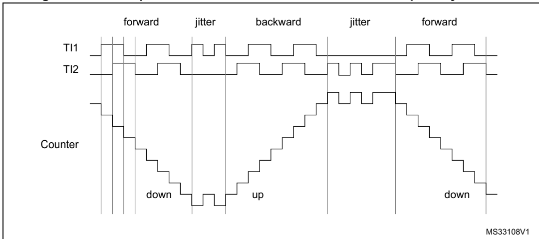
Figure 141. Example of encoder interface mode with TI1FP1 polarity inverted
