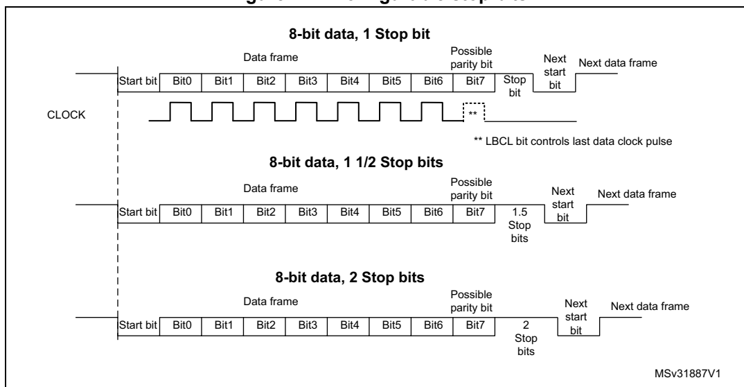
Figure 244. Configurable stop bits
