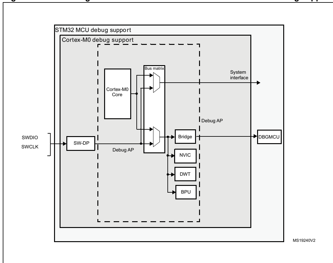
Figure 315. Block diagram of STM32L0x3 MCU and Cortex ® -M0+-level debug support
