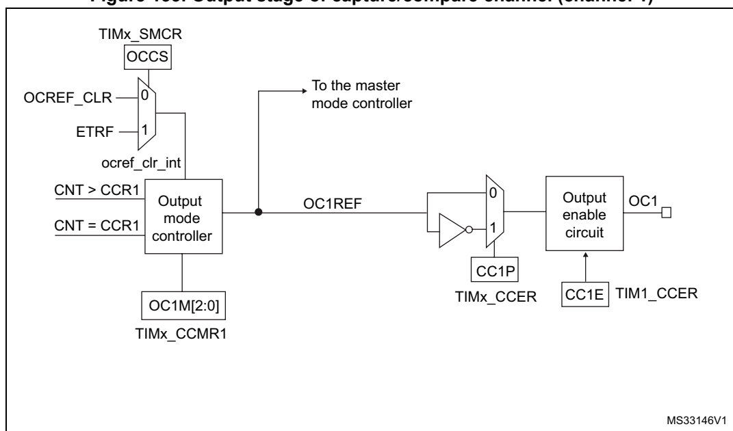
Figure 133. Output stage of capture/compare channel (channel 1)
