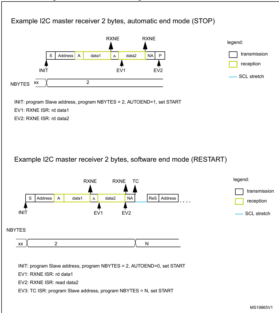
Figure 234. Transfer bus diagrams for I2C master receiver
