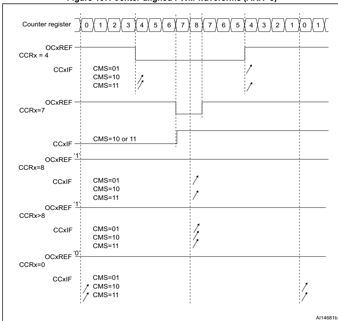
Figure 137. Center-aligned PWM waveforms (ARR=8)
