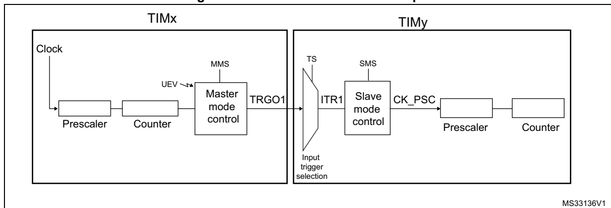
Figure 146. Master/Slave timer example
