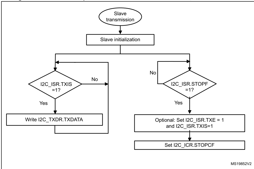
Figure 220. Transfer sequence flow for I2C slave transmitter, NOSTRETCH = 1
