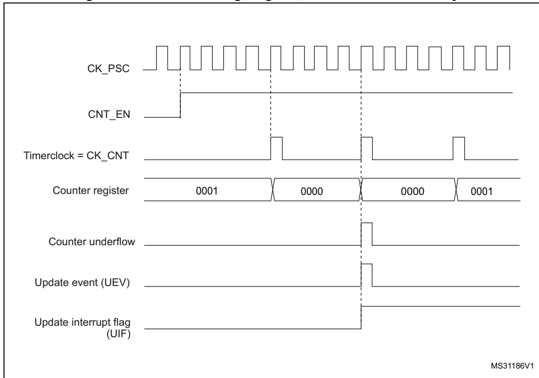
Figure 164. Counter timing diagram, internal clock divided by N
