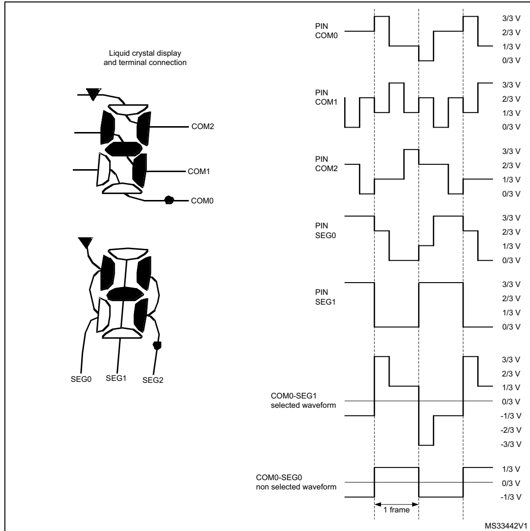
Figure 72. 1/3 duty, 1/3 bias
