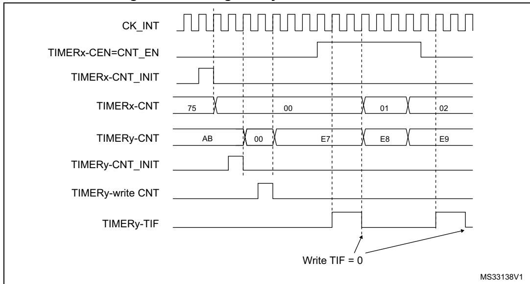
Figure 148. Gating timer y with Enable of timer x
