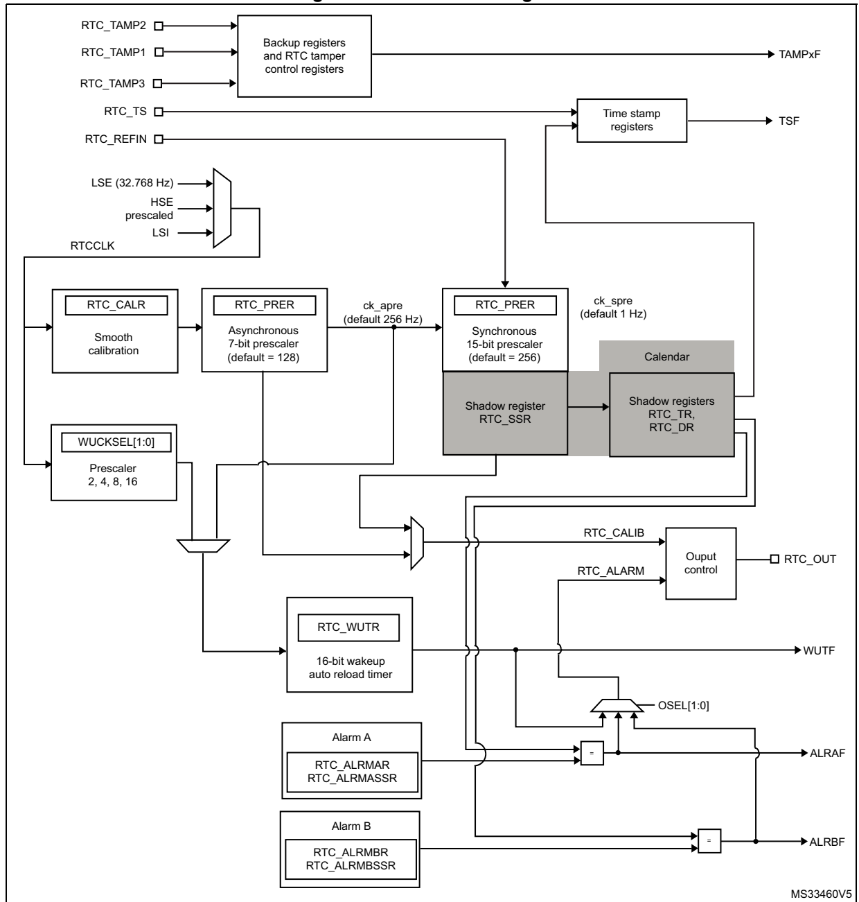
Figure 210. RTC block diagram
