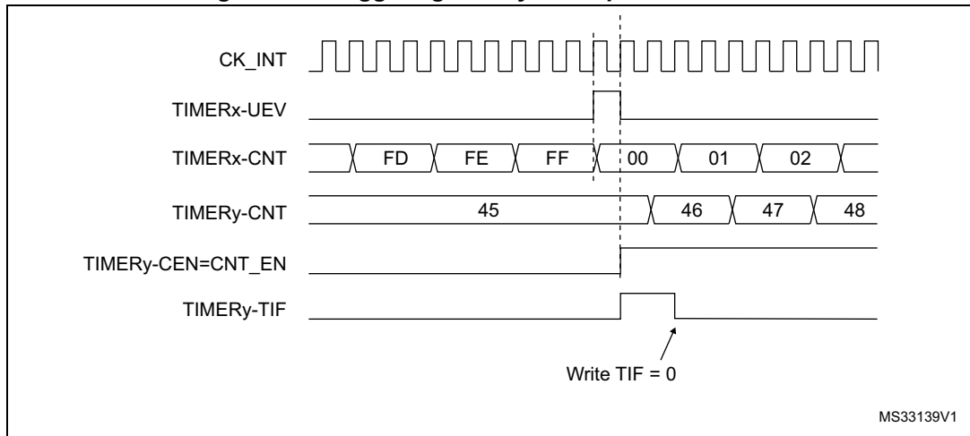
Figure 149. Triggering timer y with update of timer x
