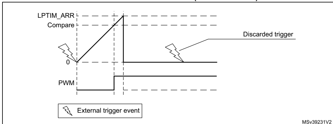
Figure 203. LPTIM output waveform, Single counting mode configuration and Set-once mode activated (WAVE bit is set)
