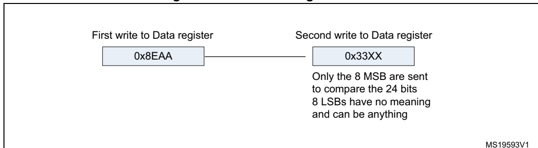
Figure 296. Transmitting 0x8EAA33
