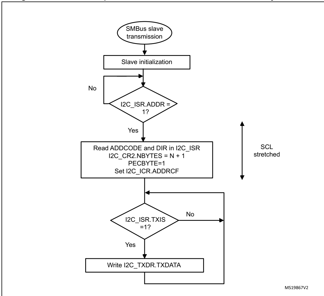
Figure 236. Transfer sequence flow for SMBus slave transmitter N bytes + PEC
