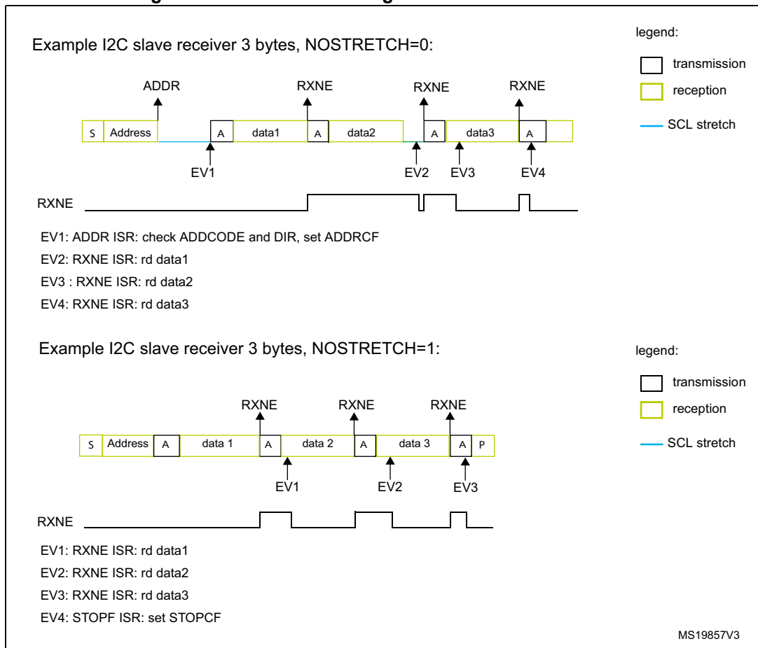
Figure 224. Transfer bus diagrams for I2C slave receiver
