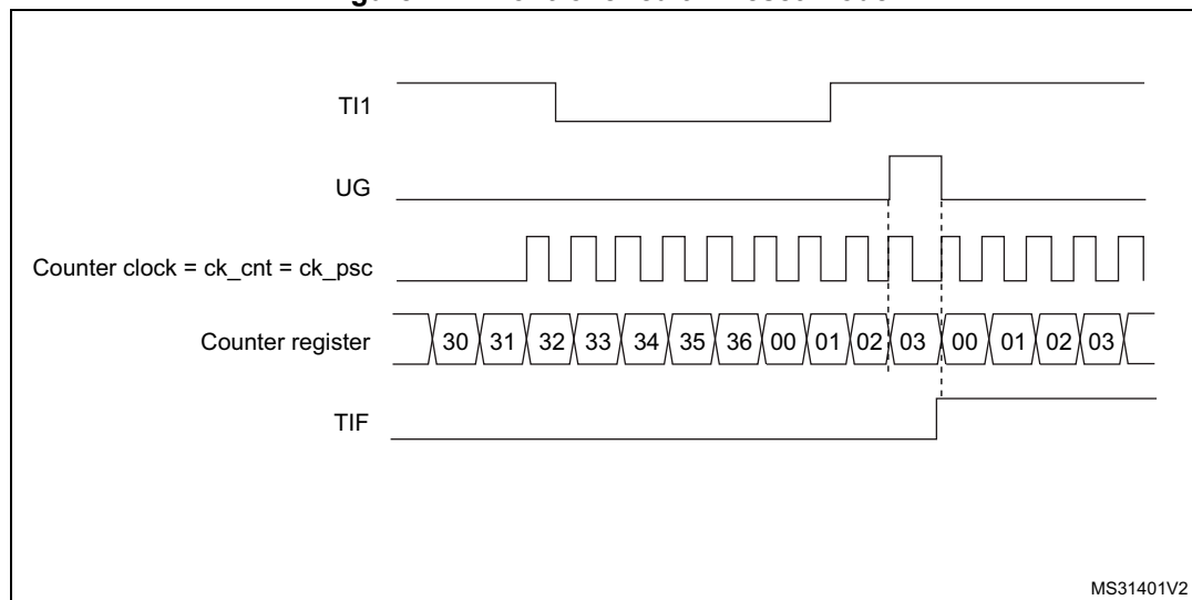
Figure 142. Control circuit in reset mode
