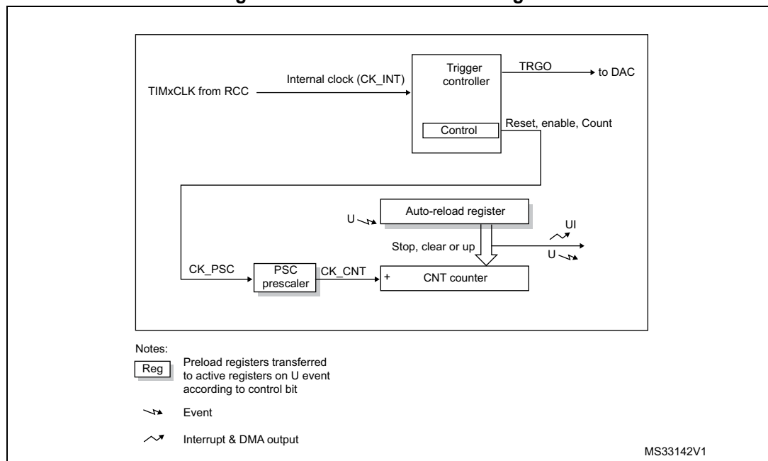
Figure 190. Basic timer block diagram
