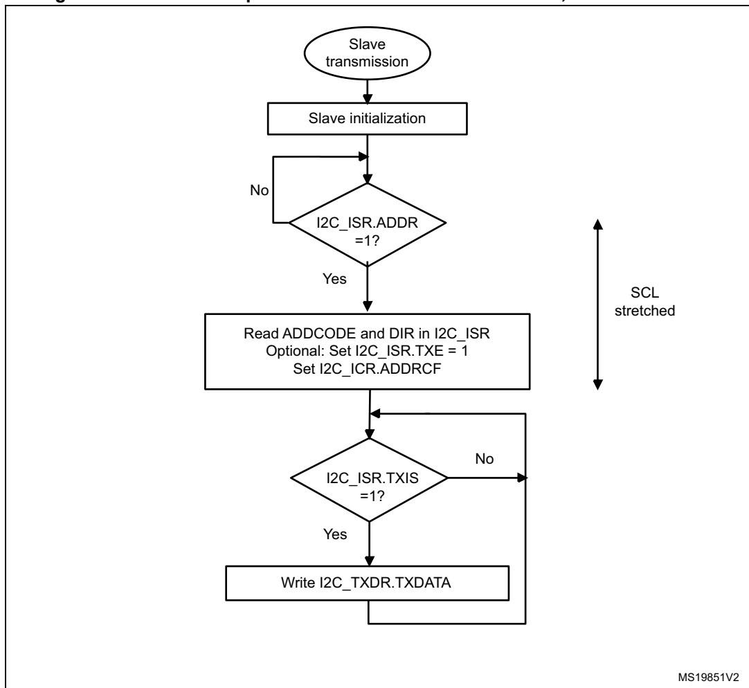
Figure 219. Transfer sequence flow for I2C slave transmitter, NOSTRETCH = 0
