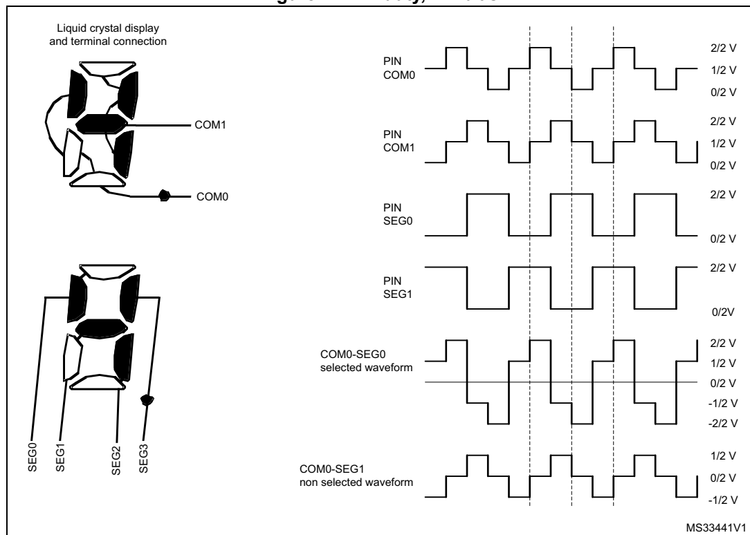
Figure 71. 1/2 duty, 1/2 bias
