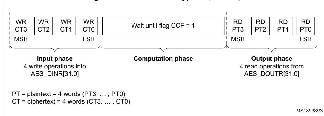
Figure 96. ECB/CBC decryption (Mode 3)
