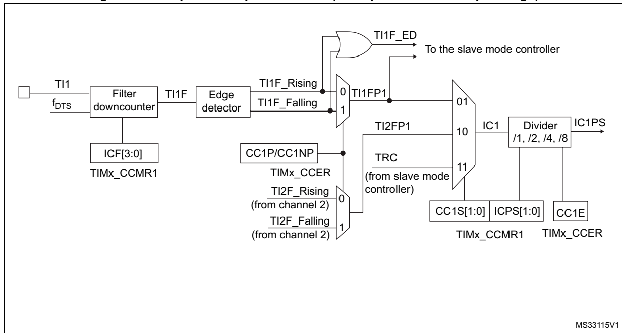
Figure 131. Capture/compare channel (example: channel 1 input stage)
