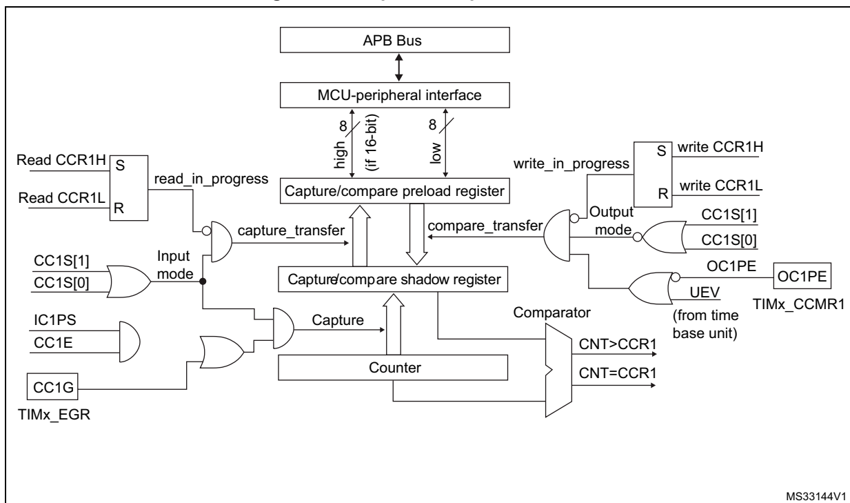
Figure 132. Capture/compare channel 1 main circuit
