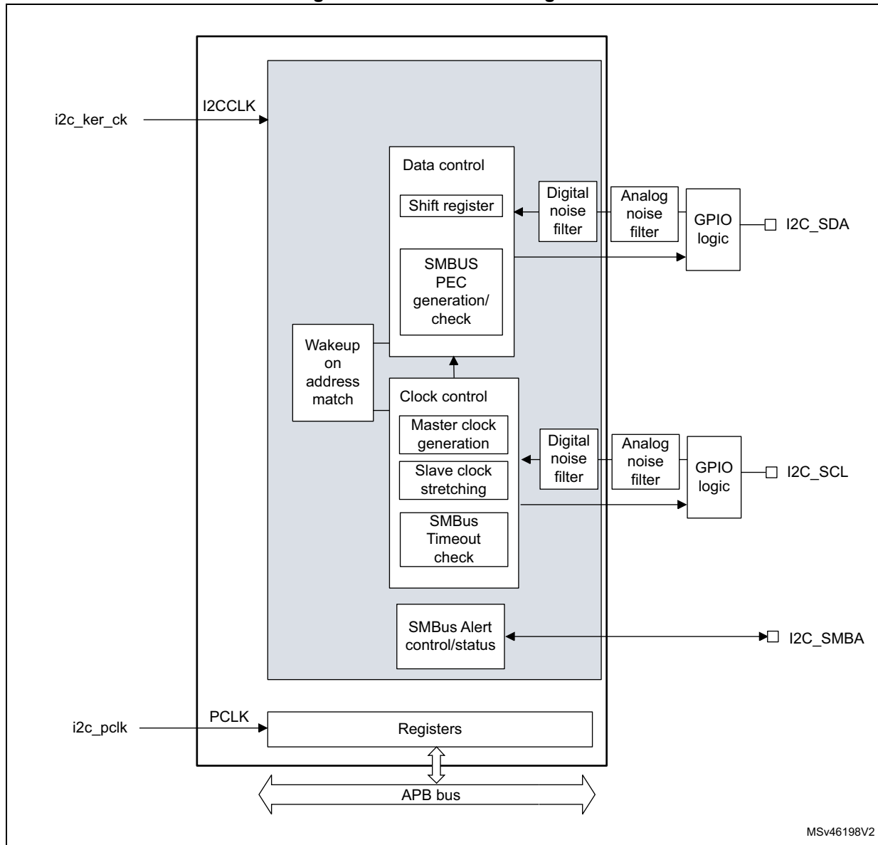
Figure 211. I2C1/3 block diagram
