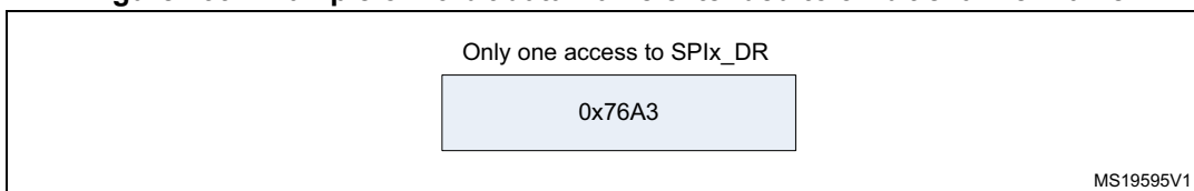
Figure 299. Example of 16-bit data frame extended to 32-bit channel frame
