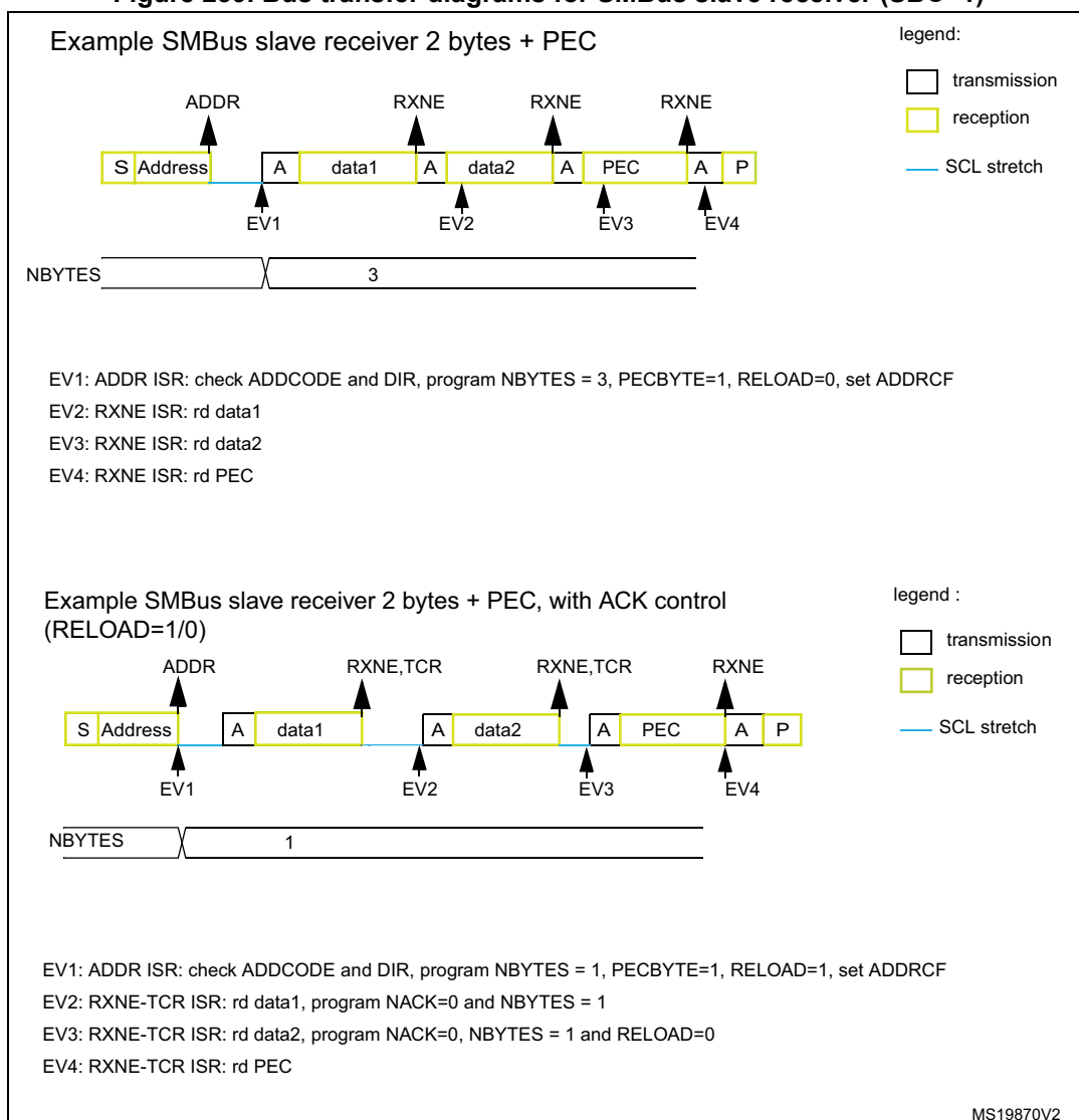
Figure 239. Bus transfer diagrams for SMBus slave receiver (SBC=1)
