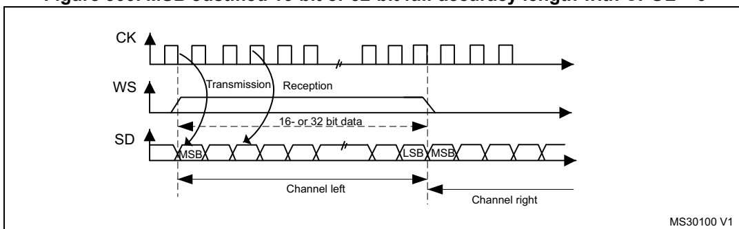
Figure 300. MSB Justified 16-bit or 32-bit full-accuracy length with CPOL = 0
