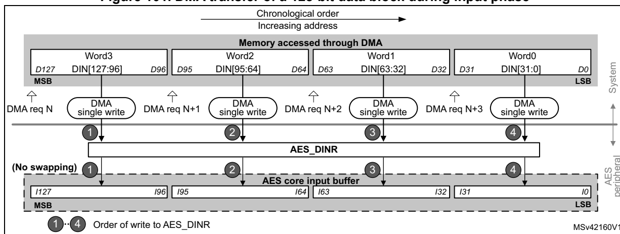
Figure 101. DMA transfer of a 128-bit data block during input phase
