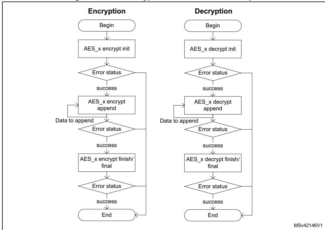
Figure 88. STM32 cryptolib AES flowchart example
