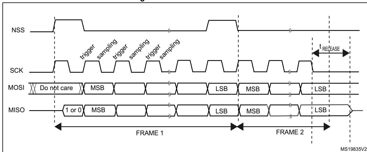
Figure 291. TI mode transfer
