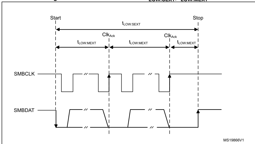
Figure 235. Timeout intervals for t_{LOW:SEXT} , t_{LOW:MEXT}
