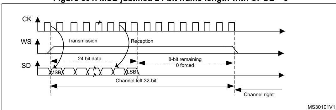
Figure 301. MSB justified 24-bit frame length with CPOL = 0
