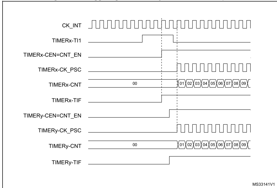
Figure 151. Triggering timer x and y with timer x TI1 input
