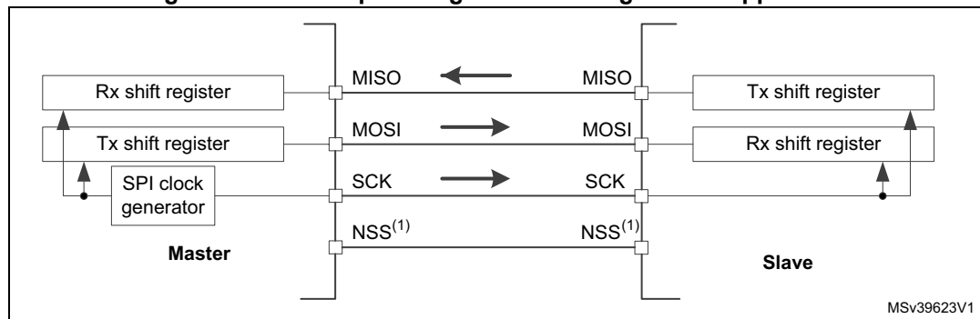
Figure 280. Full-duplex single master/ single slave application
