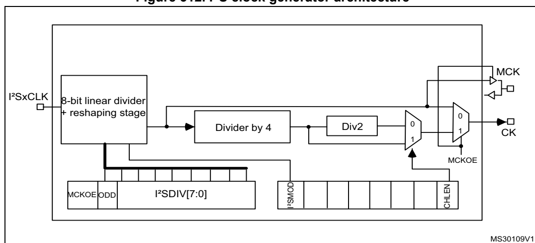
Figure 312. I 2 S clock generator architecture
