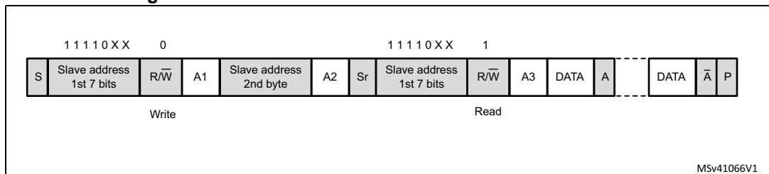
Figure 227. 10-bit address read access with HEAD10R = 0
