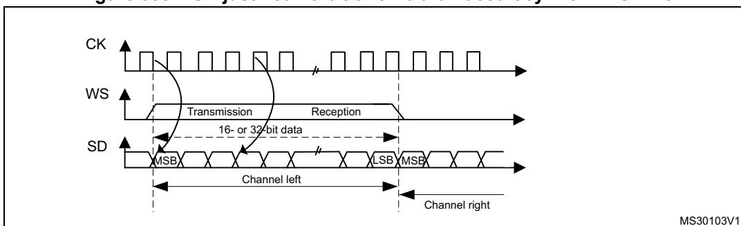
Figure 303. LSB justified 16-bit or 32-bit full-accuracy with CPOL = 0
