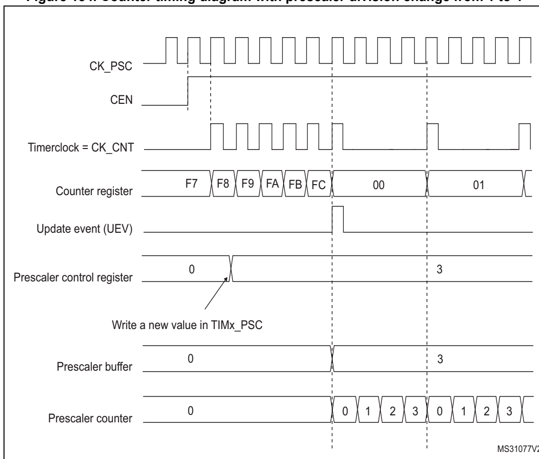
Figure 154. Counter timing diagram with prescaler division change from 1 to 4
