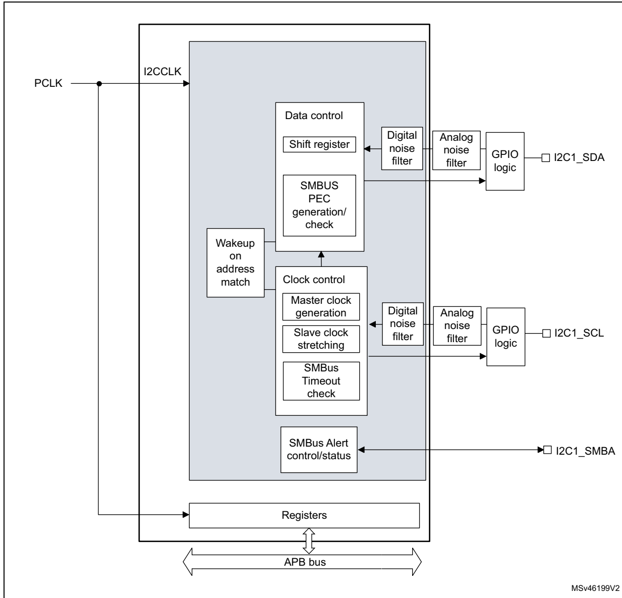
Figure 212. I2C2 block diagram
