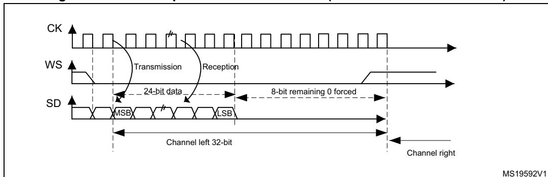
Figure 295. I 2 S Philips standard waveforms (24-bit frame with CPOL = 0)
