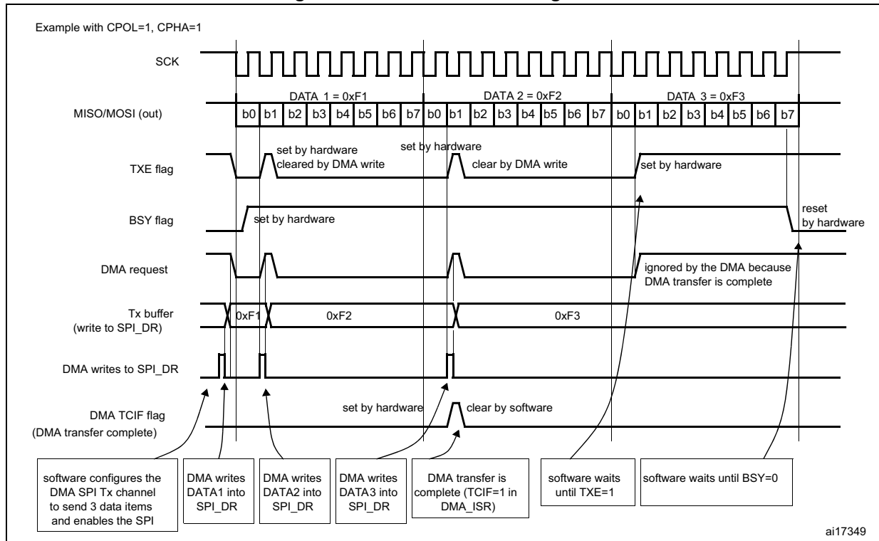
Figure 289. Transmission using DMA
