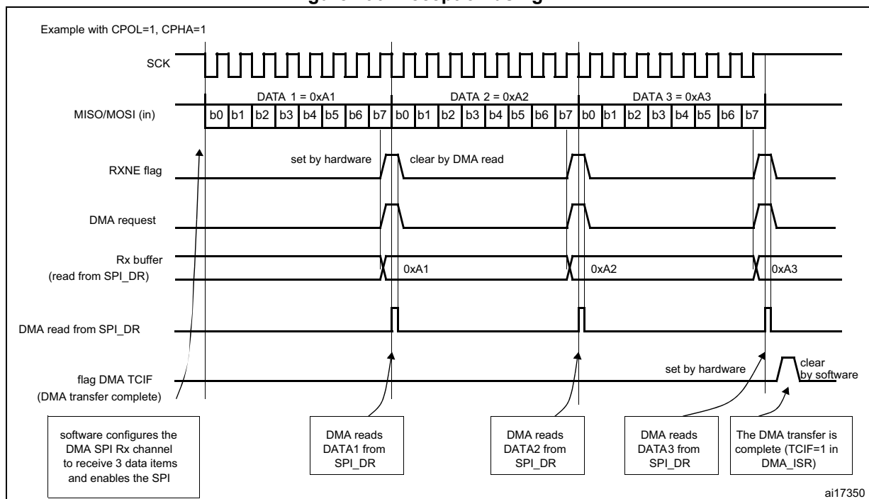
Figure 290. Reception using DMA
