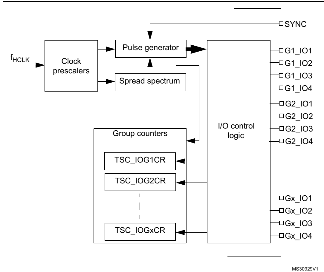
Figure 79. TSC block diagram
