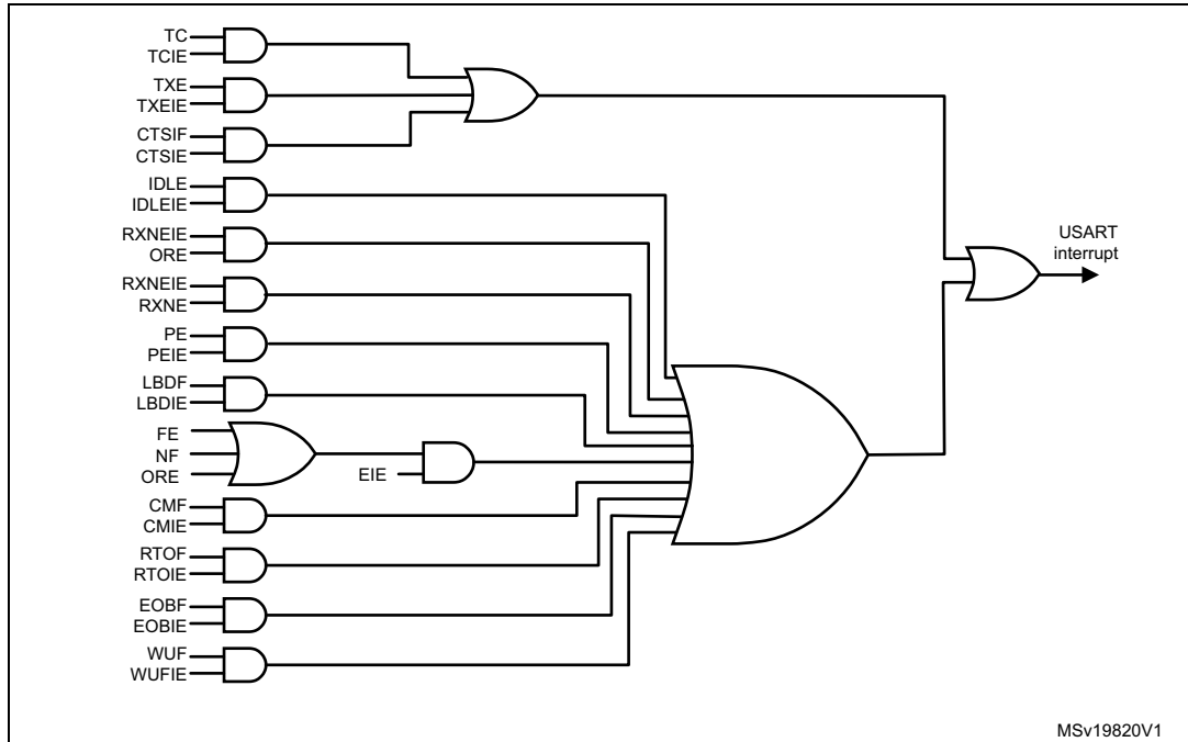
Figure 266. USART interrupt mapping diagram
