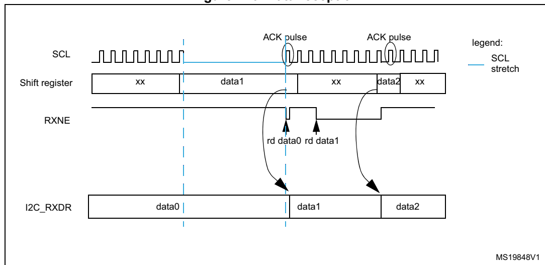
Figure 216. Data reception
