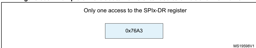
Figure 308. Example of 16-bit data frame extended to 32-bit channel frame
