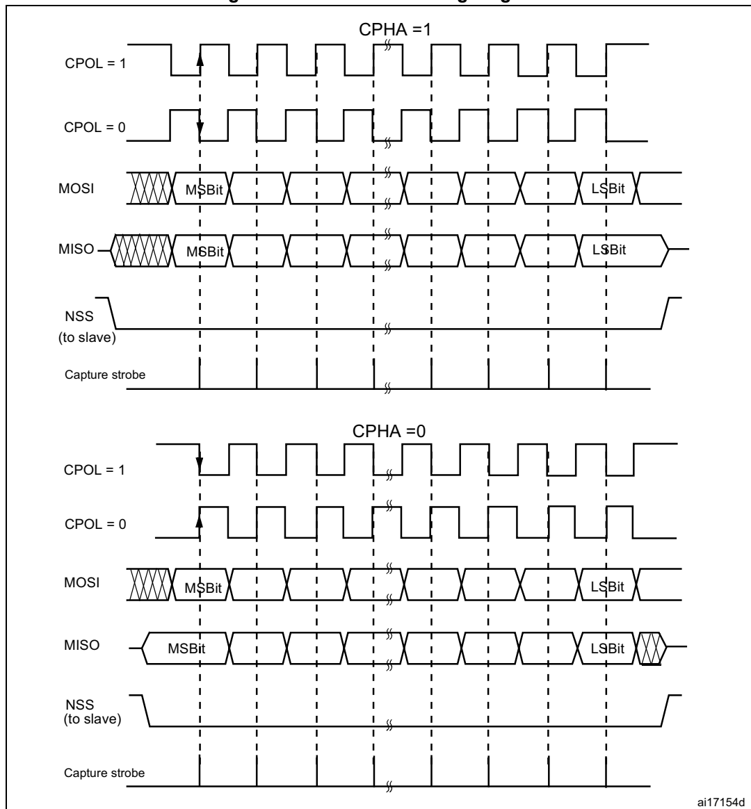
Figure 286. Data clock timing diagram
