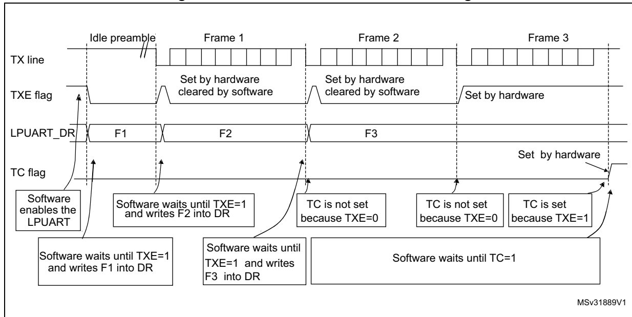
Figure 270. TC/TXE behavior when transmitting
