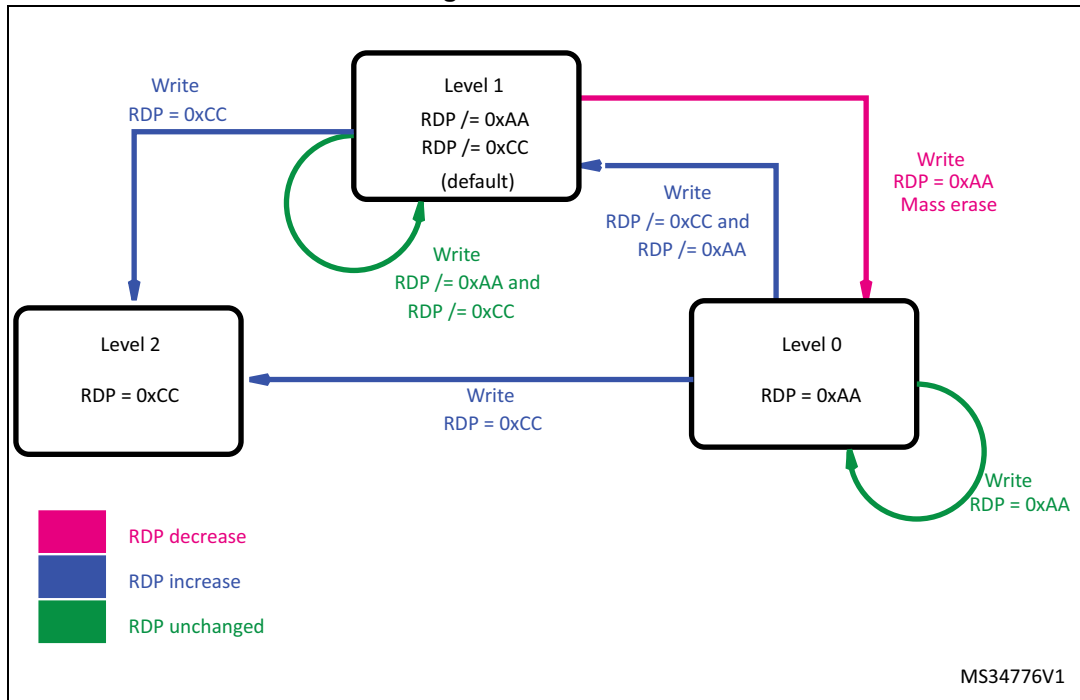
Figure 6. RDP levels
