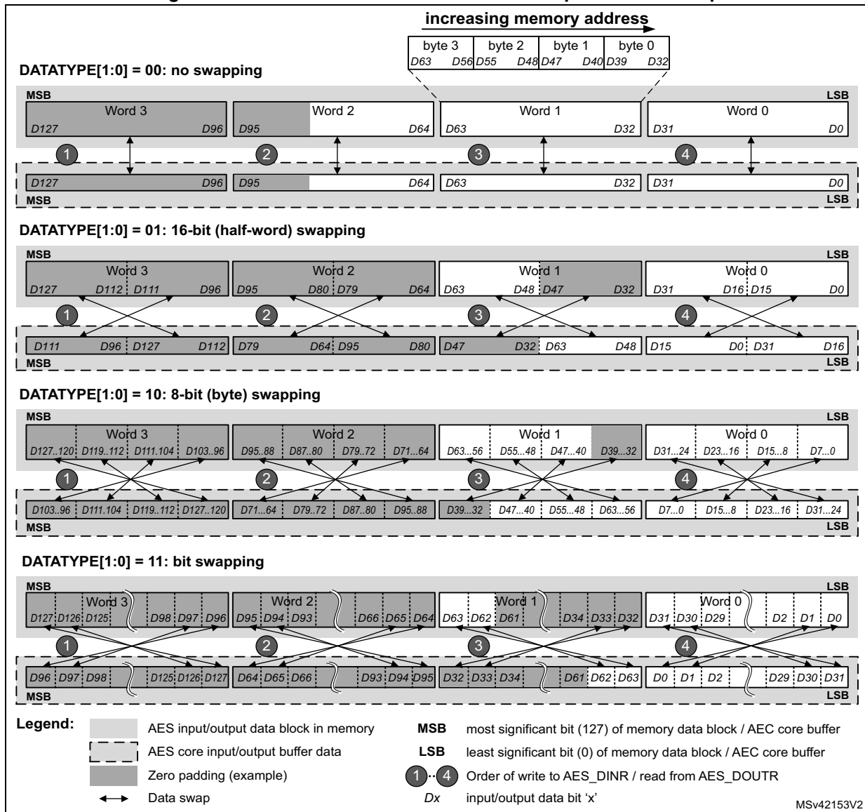
Figure 100. 128-bit block construction with respect to data swap
