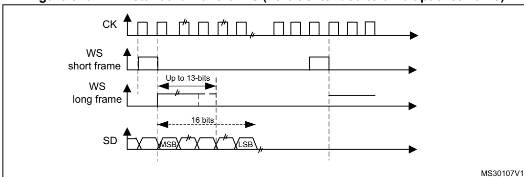
Figure 310. PCM standard waveforms (16-bit extended to 32-bit packet frame)
