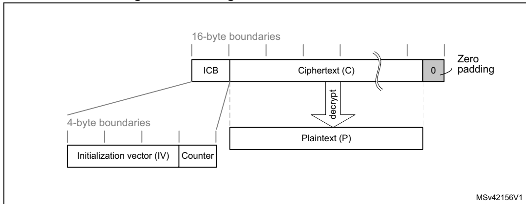
Figure 97. Message construction in CTR mode
