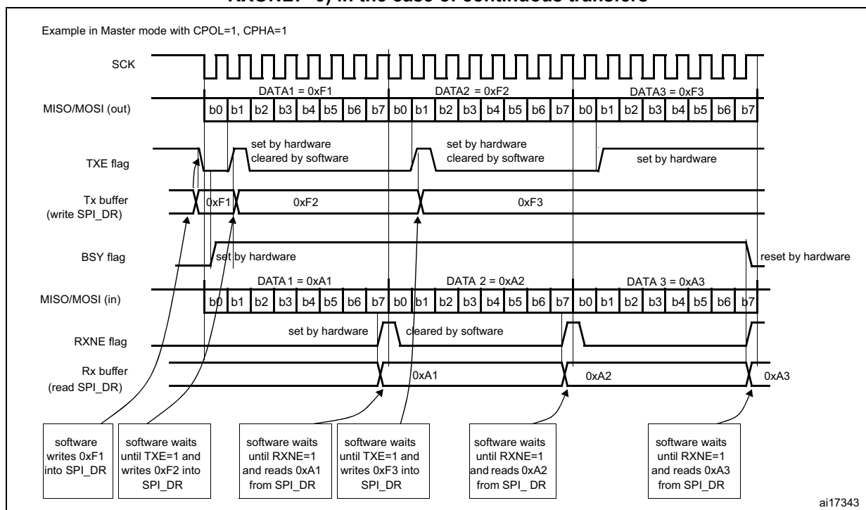
Figure 287. TXE/RXNE/BSY behavior in master / full-duplex mode (BIDIMODE=0, RXONLY=0) in the case of continuous transfers
