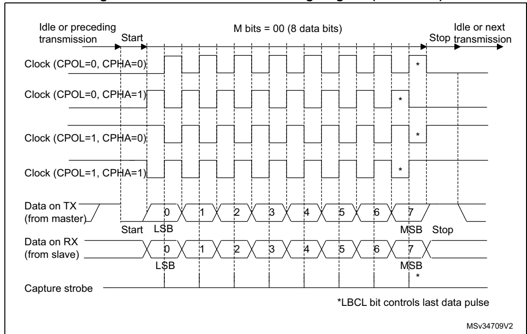
Figure 254. USART data clock timing diagram (M bits = 00)
