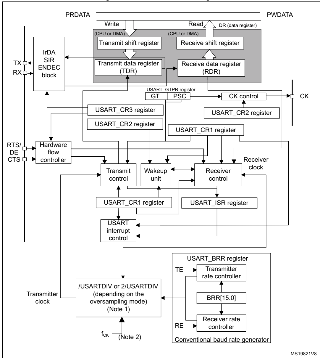
Figure 242. USART block diagram
