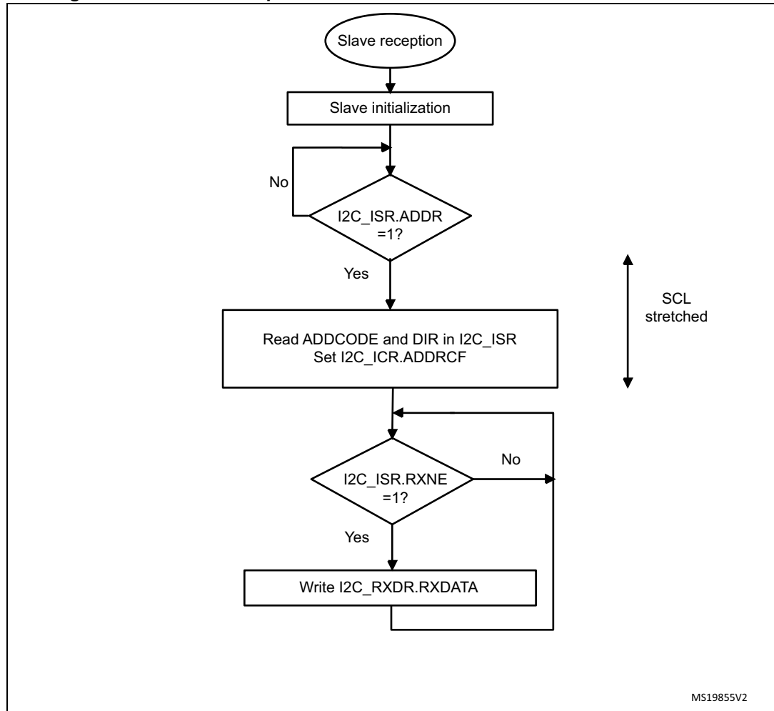
Figure 222. Transfer sequence flow for slave receiver with NOSTRETCH = 0
