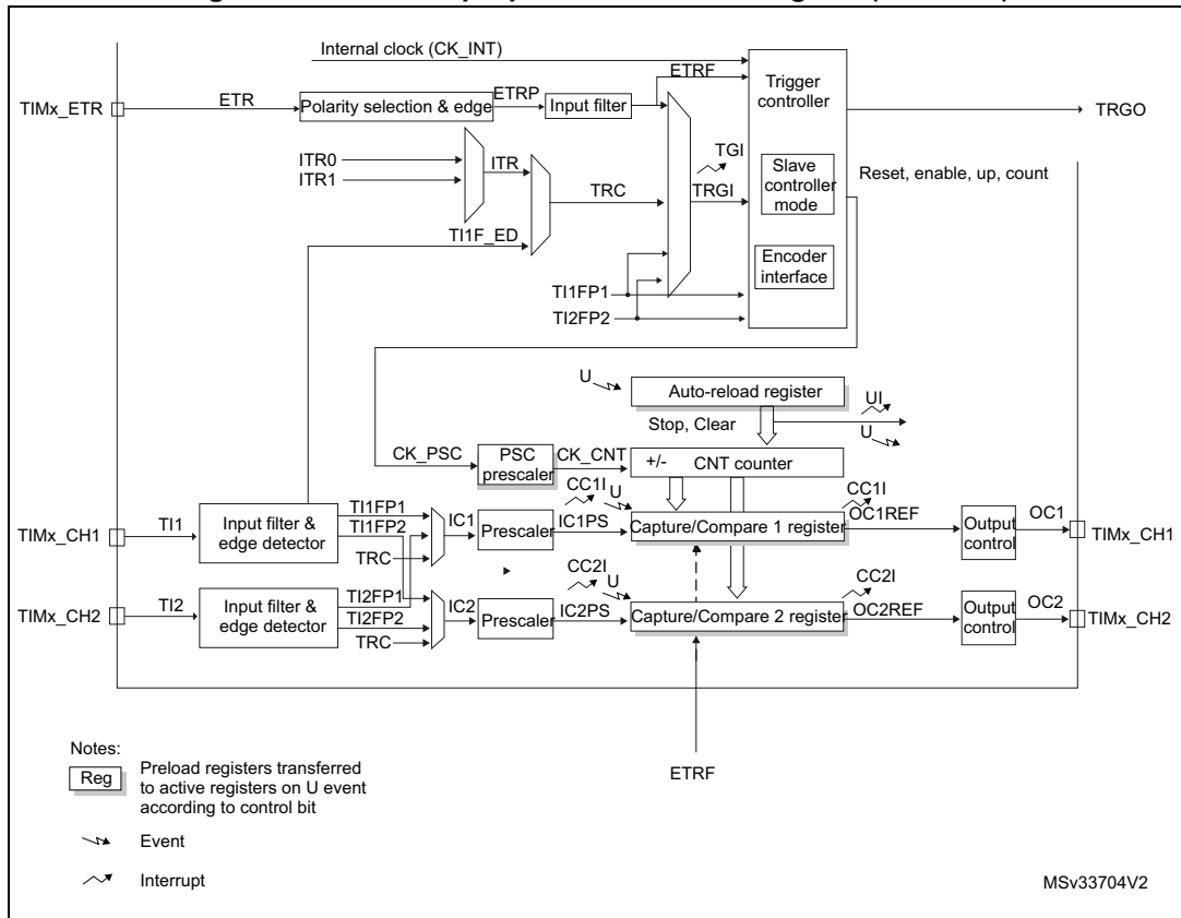
Figure 152. General-purpose timer block diagram (TIM21/22)
