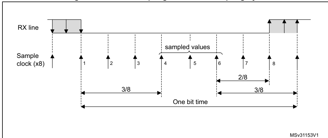
Figure 248. Data sampling when oversampling by 8
