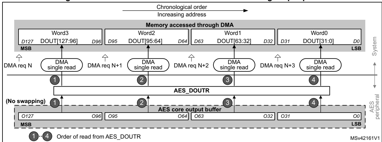
Figure 102. DMA transfer of a 128-bit data block during output phase
