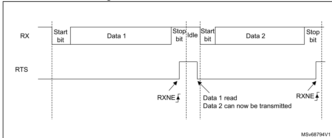
Figure 276. RS232 RTS flow control
