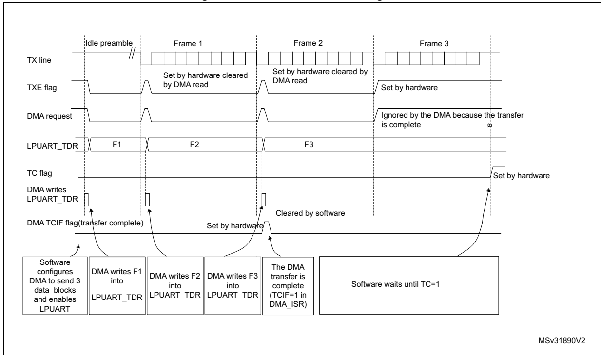
Figure 273. Transmission using DMA
