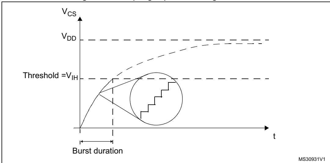
Figure 81. Sampling capacitor voltage variation
