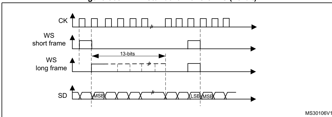
Figure 309. PCM standard waveforms (16-bit)
