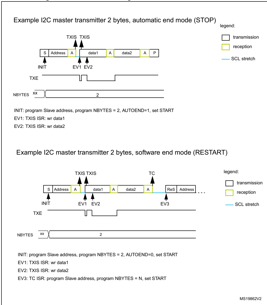
Figure 231. Transfer bus diagrams for I2C master transmitter
