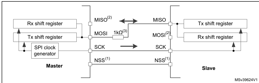
Figure 281. Half-duplex single master/ single slave application
