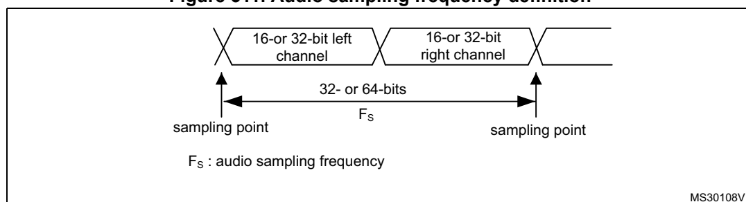
Figure 311. Audio sampling frequency definition
