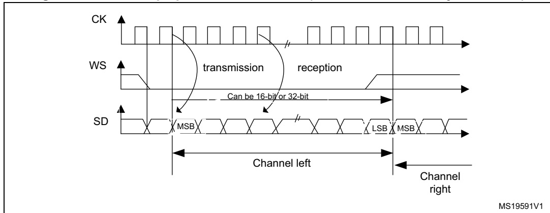
Figure 294. I 2 S Philips protocol waveforms (16/32-bit full accuracy, CPOL = 0)
