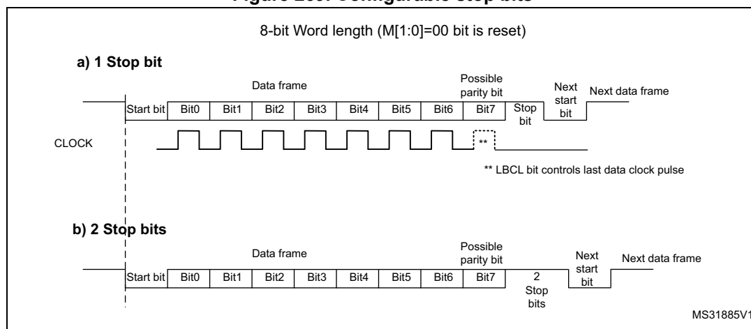
Figure 269. Configurable stop bits
