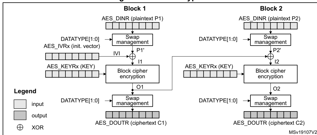
Figure 93. CBC encryption
