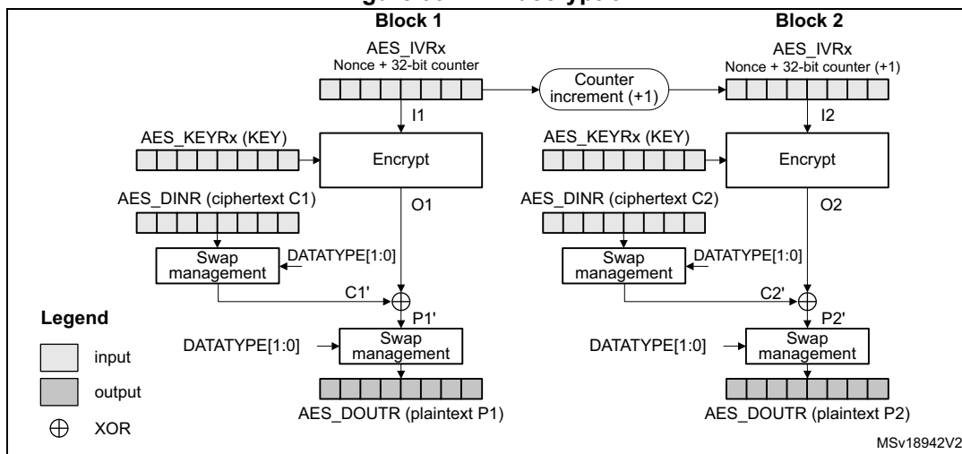
Figure 99. CTR decryption
