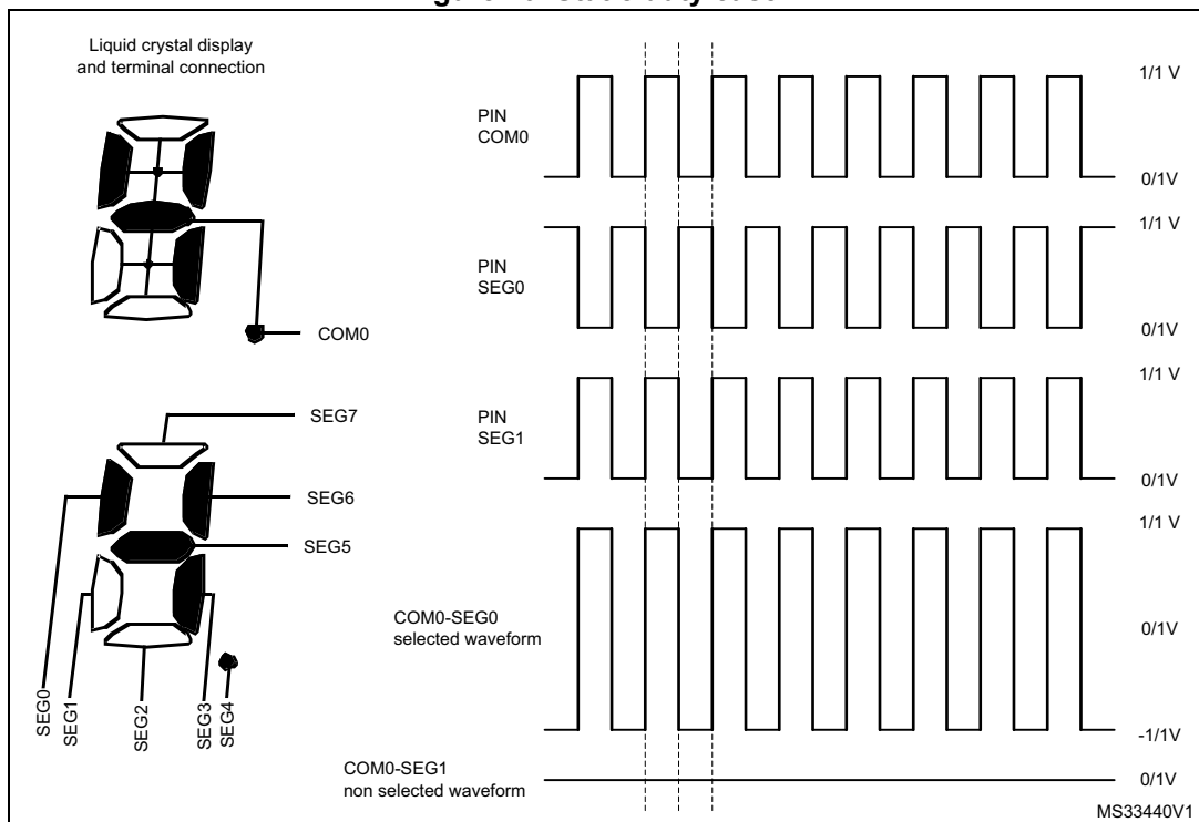
Figure 70. Static duty case 2
