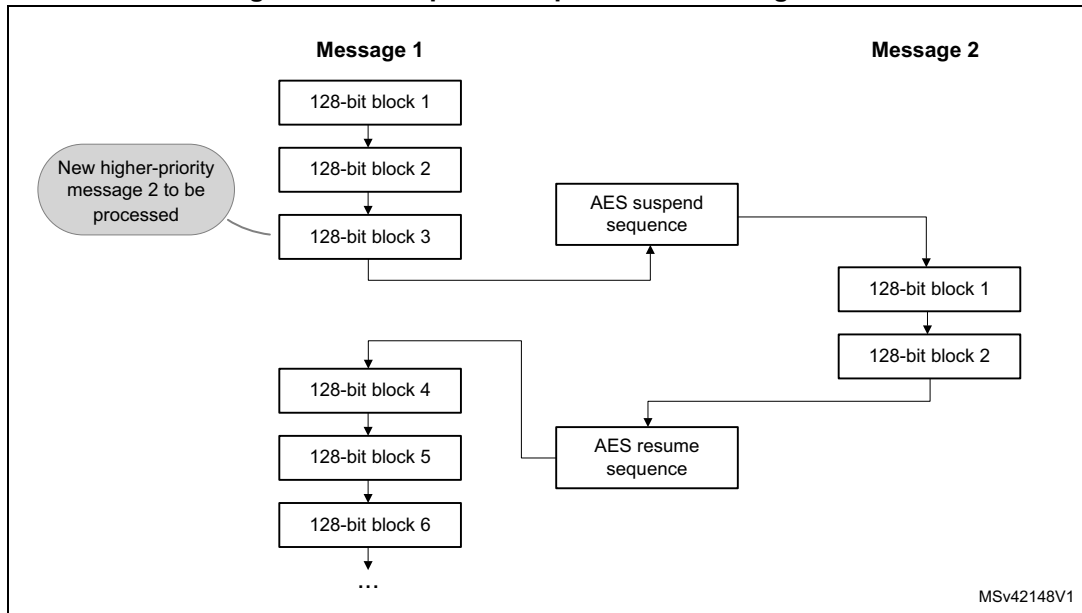
Figure 90. Example of suspend mode management
