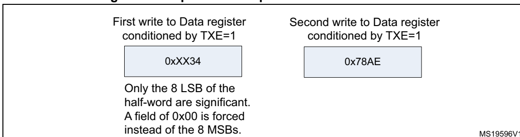
Figure 305. Operations required to transmit 0x3478AE
