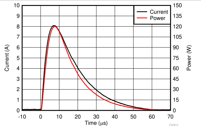
Figure 6-6. Positive Surge Waveform (8/20 \mu s)
