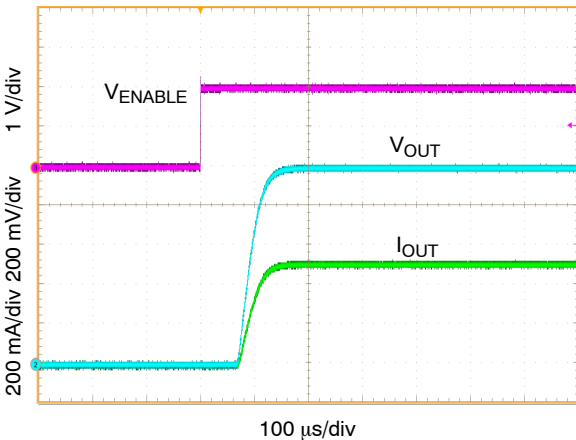
Figure 16. Enable Turn-on Response, Output Resistive Load 500 mA, C_{OUT} = 10\text{ }\mu\text{F}
