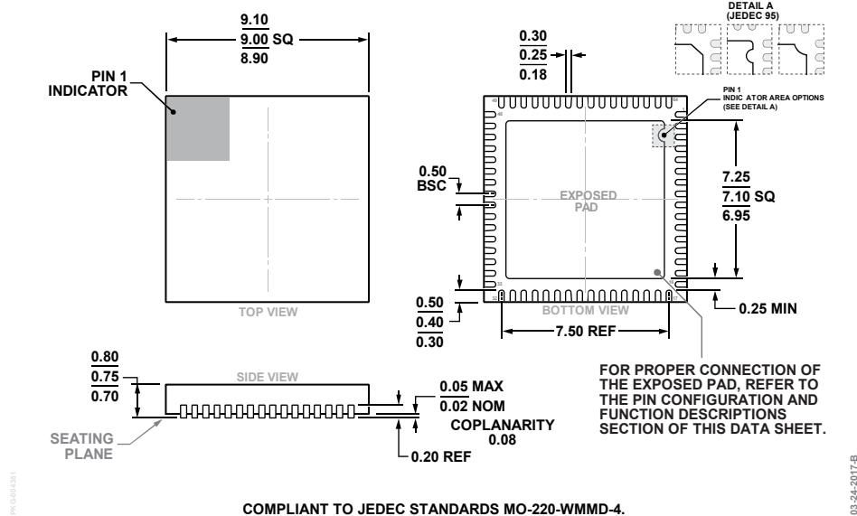
Figure 87. 64-Lead Lead Frame Chip Scale Package [LFCSP] 9 mm × 9 mm Body and 0.75 mm Package Height (CP-64-12) Dimensions shown in millimeters
