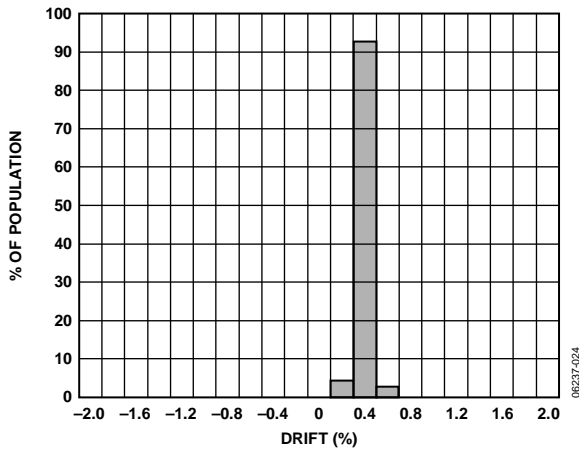
Figure 24. X-Axis Sensitivity Drift Over Temperature, V_s = 5V
