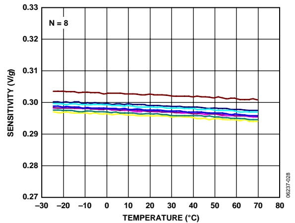
Figure 28. Y-Axis Sensitivity vs. Temperature Eight Parts Soldered to PCB, V_s = 3V
