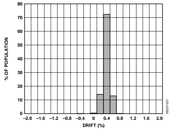
Figure 27. Y-Axis Sensitivity Drift Over Temperature, V_s = 5V
